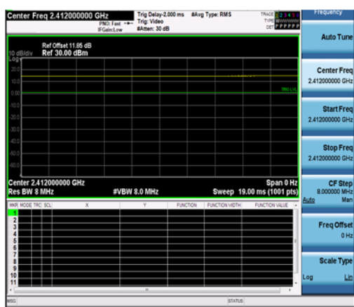
NTNV-11G-2412
