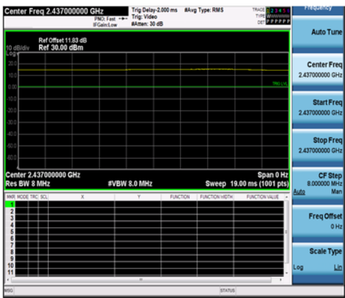
NTNV-11AX20SISO-2437
