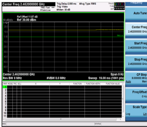
NTNV-11AX20SISO-2462
