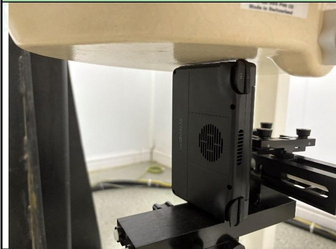
Photo 10: Bottom side 0mm(Close)
