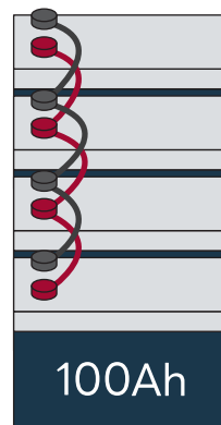
Parallel Connection 24V(25.6V) 400Ah
