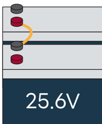
Series Connection 48V(51.2V) 100Ah
