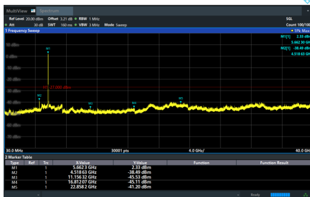
11ac (HT20) CH120
