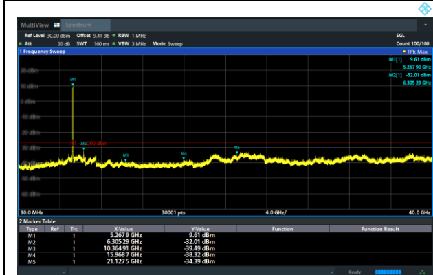
11ax (HE40) CH54
