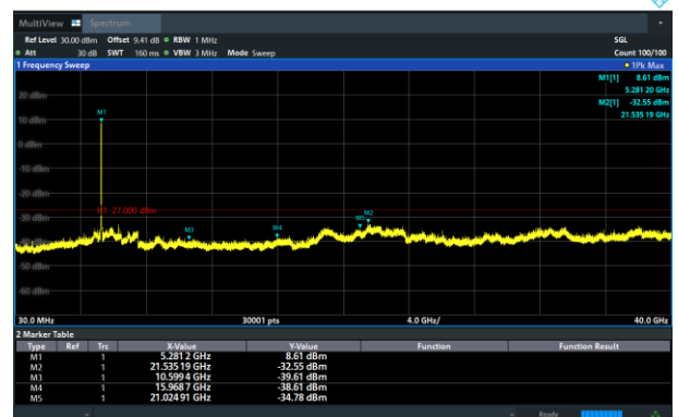
11ac (HT40) CH54
