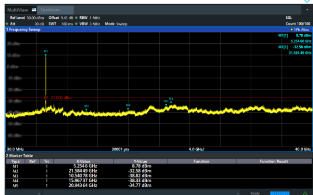
11ac (HT20) CH52
