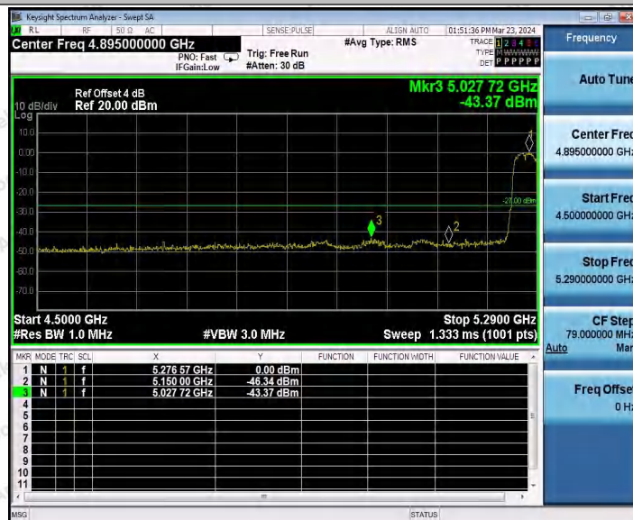
11N40SISO_Ant1_High_5310
