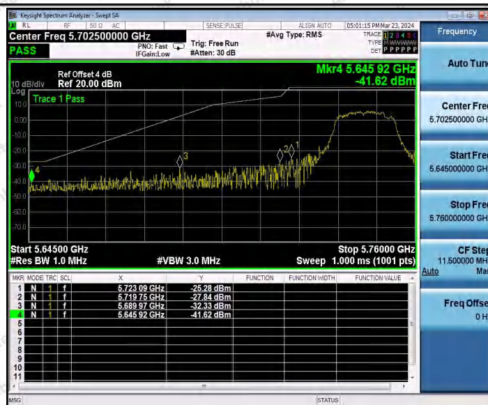
11AC20SISO_Ant2_Low_5745
