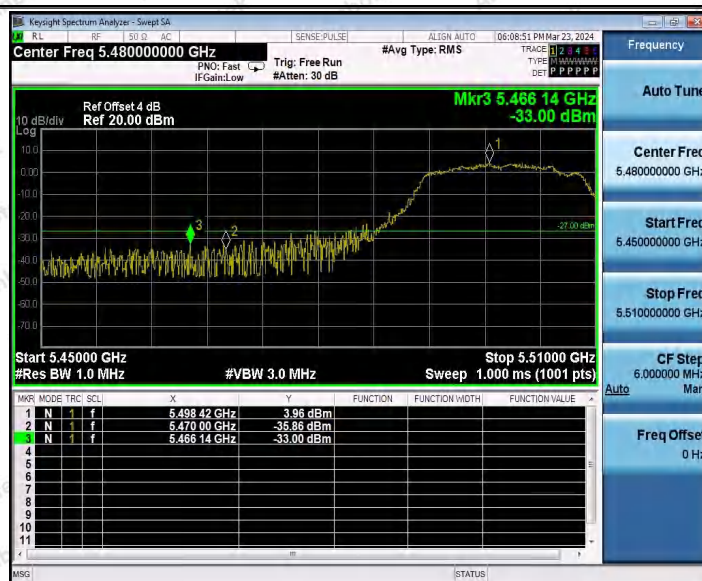
11AC20SISO_Ant2_Low_5500
