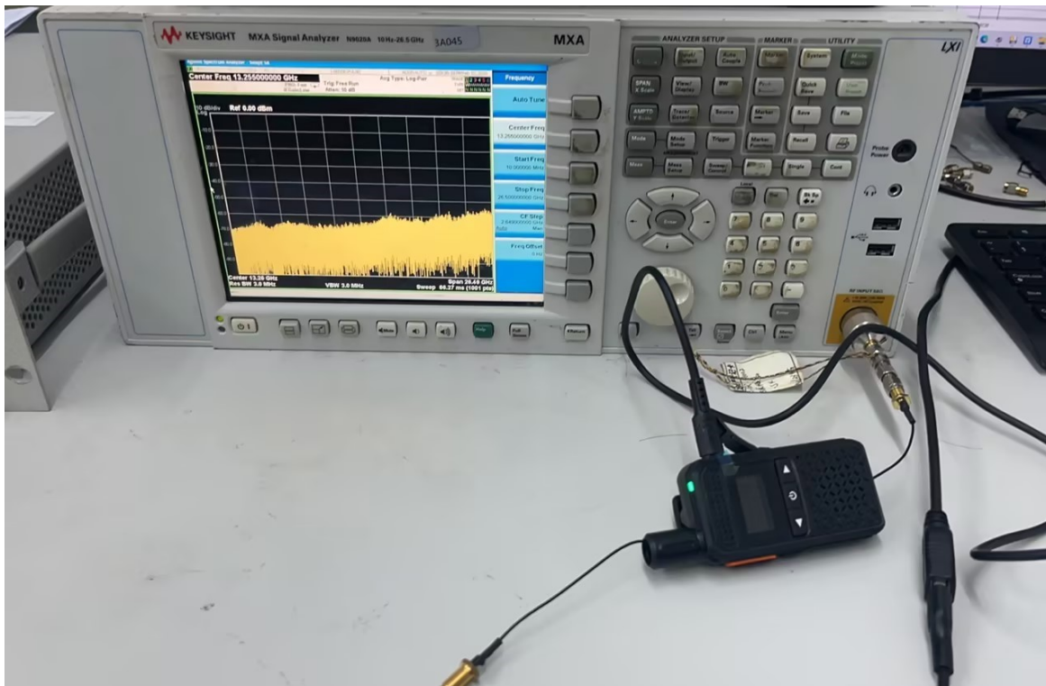
BT Conducted Test Setup
