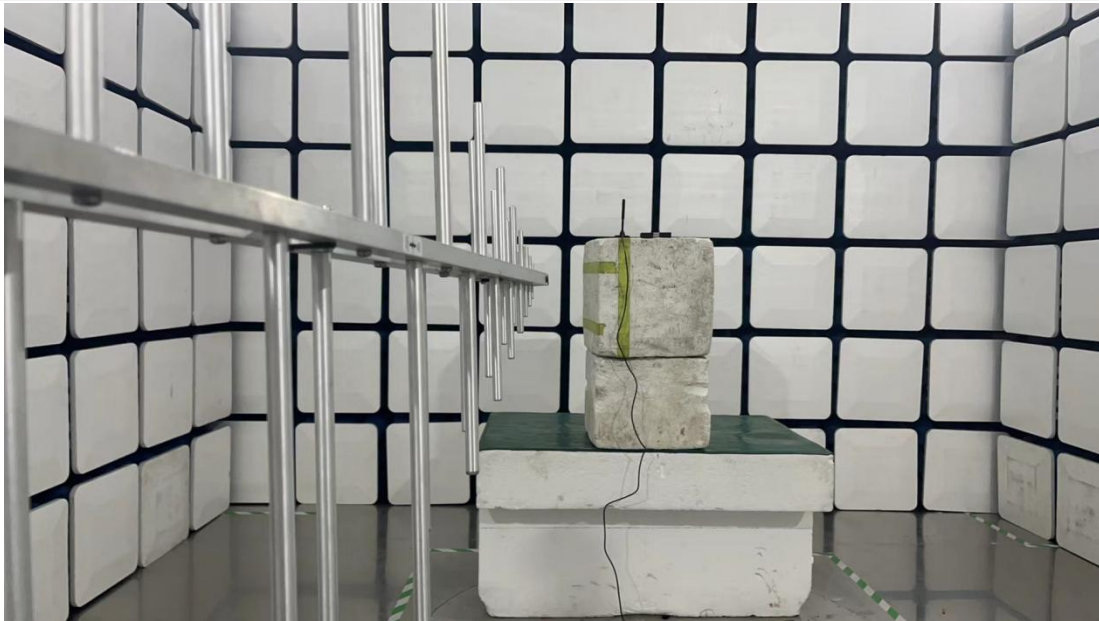
30MHz-1GHz-RF
