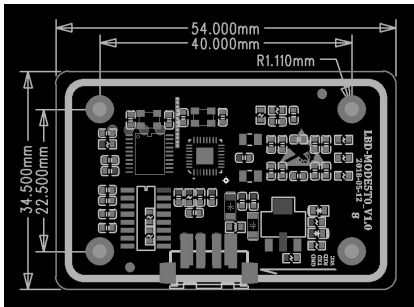
Panel Mount Dimensions
