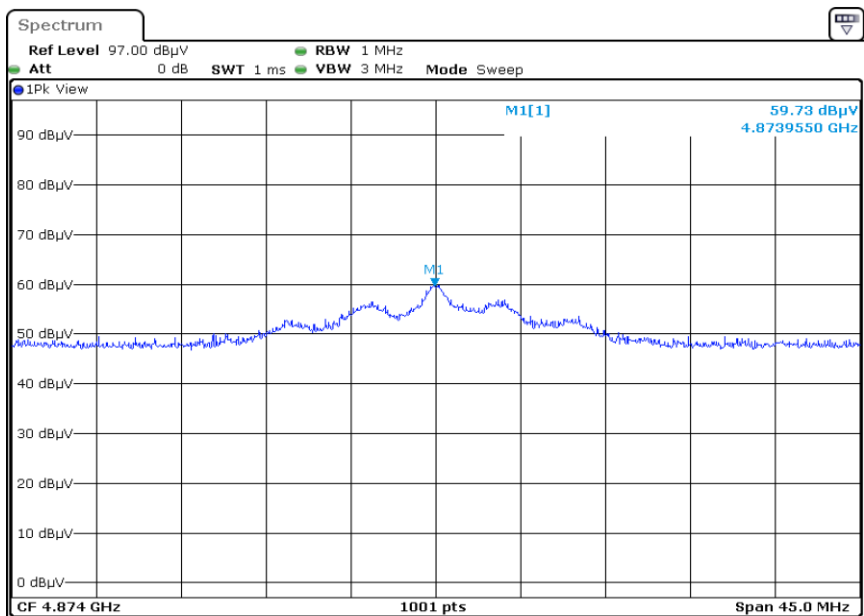
F2 X2 4874.0 Harmonic Vertical PEAK
