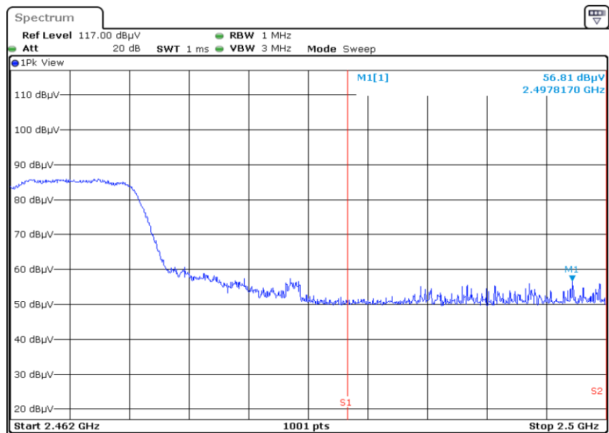
2462.0 F3 RestrictedBand Vertical PEAK
