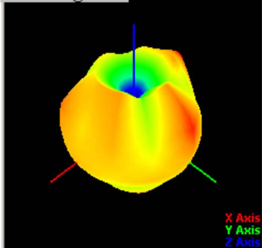
5275.00MHz@T45P45
