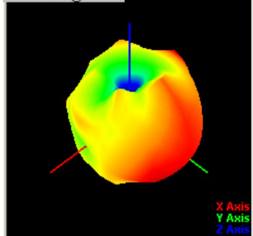
5350.00MHz@T45P45
