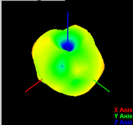
5350.00MHz@T45P45
