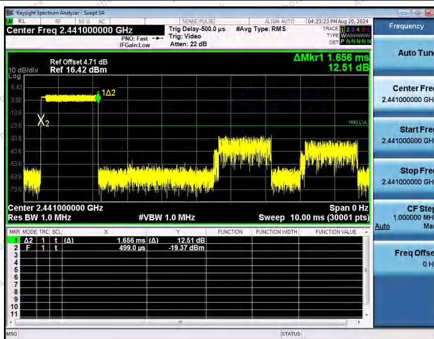
Dwell_Time_(Hopping)_NVNT_ANT1_2-DH3_2441_00_Accumulated
