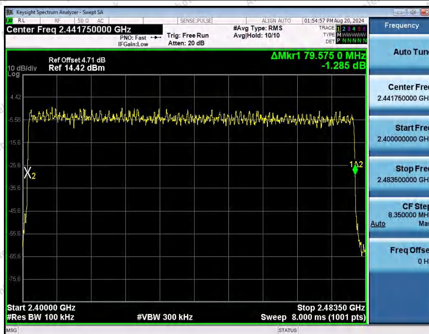
Number_of_Hopping_Channel_(Hopping)_NVNT_ANT1_3-DH5_Hopping
