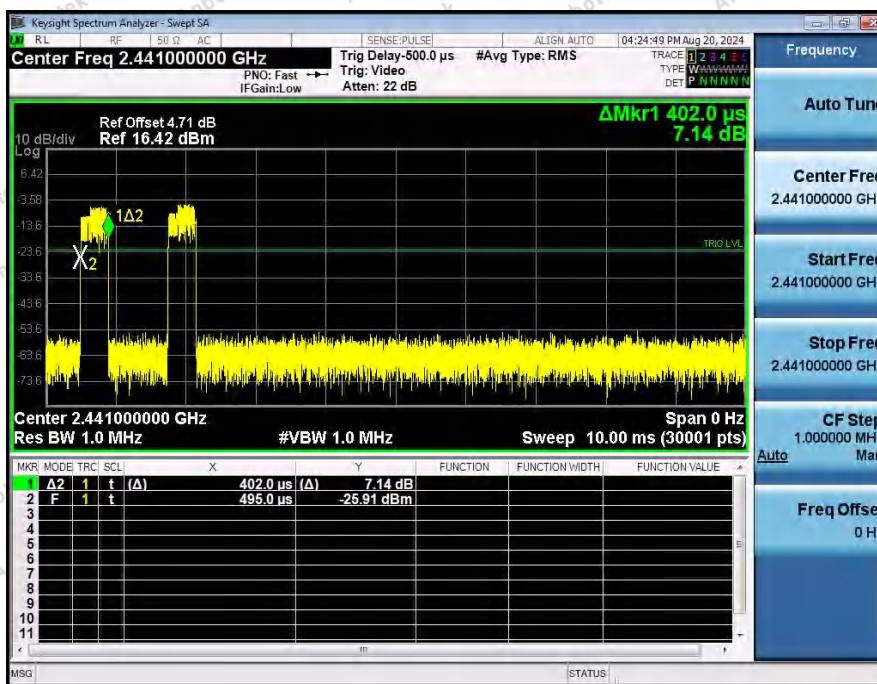
Dwell_Time_(Hopping)_NVNT_ANT1_3-DH1_2441_00_Accumulated
