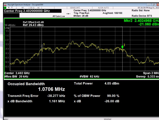
\pi/4 DQPSK_2-DH1_Channel 0
