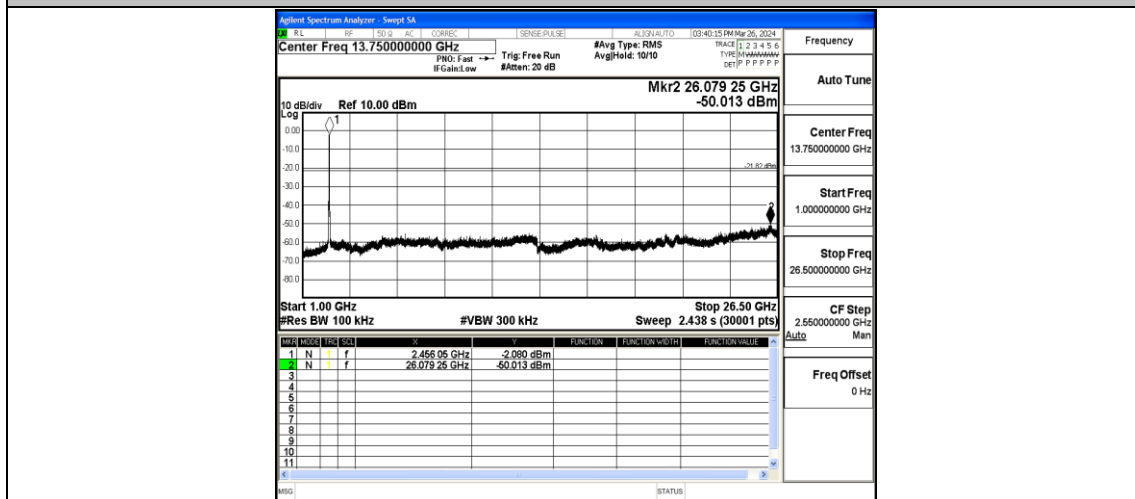
11N40SISO-Ant1-2452-1000~26500-PASS
