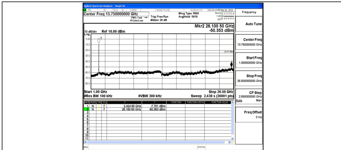
11N40SISO-Ant1-2437-1000~26500-PASS
