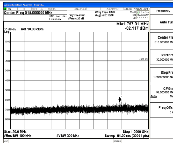
11N20SISO-Ant1-2462-30~1000-PASS
