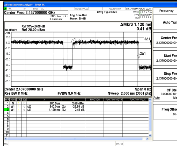
NTNV-11N40SISO-Ant1-2437
