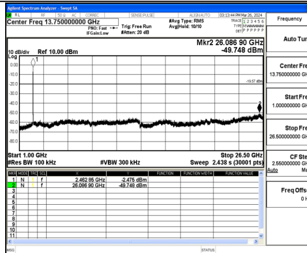
11N20SISO-Ant1-2462-1000~26500-PASS
