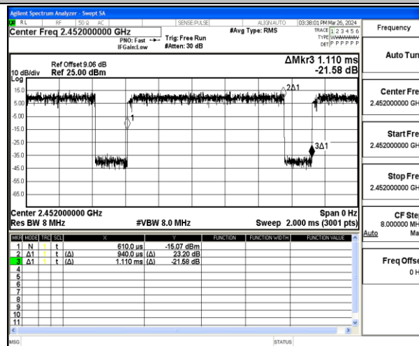
NTNV-11N40SISO-Ant1-2452
