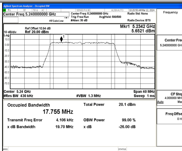
11AC20MIMO-Ant1-5240
