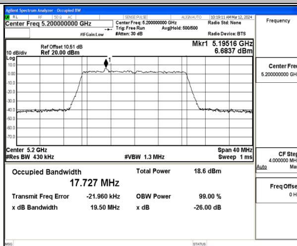
11AC20MIMO-Ant2-5200
