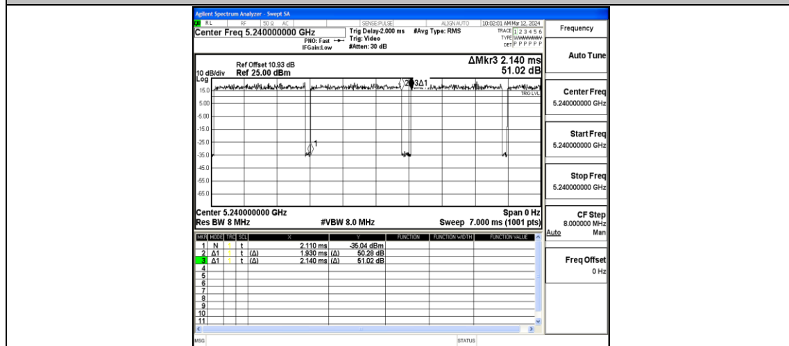
NTNV-11N20MIMO-Ant2-5240
