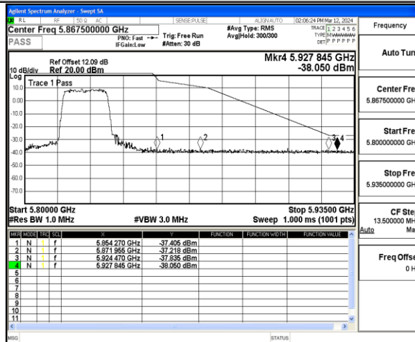
11AC20MIMO-Ant1-5825-PASS
