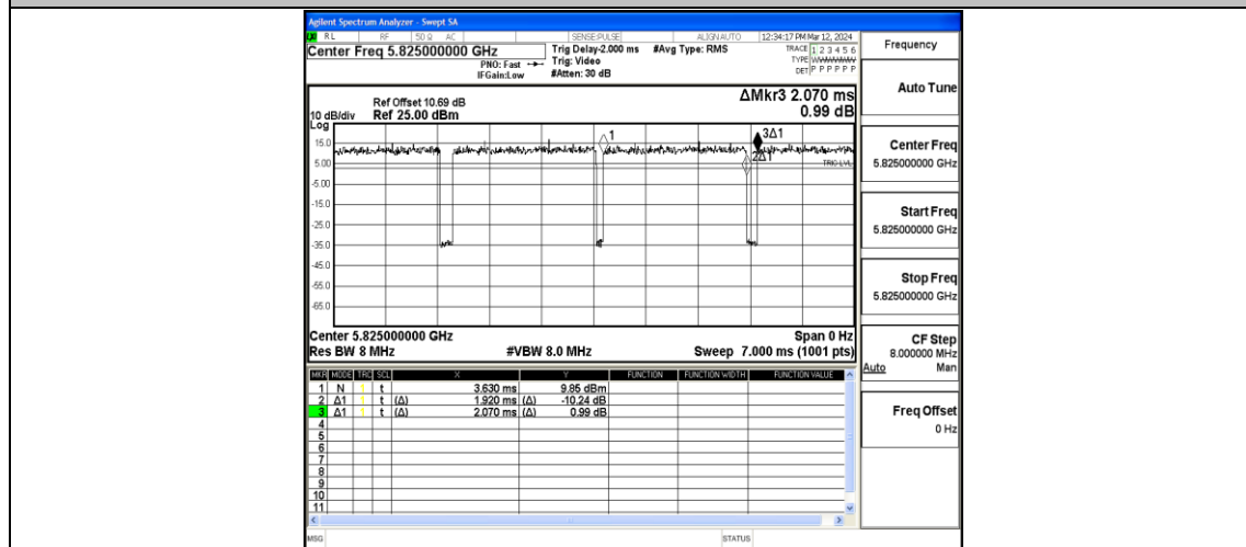
NTNV-11N20MIMO-Ant2-5825
