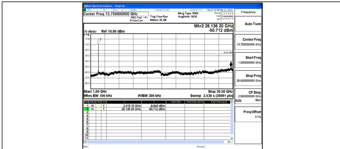
11N40MIMO-Ant2-2422-1000~26500-PASS
