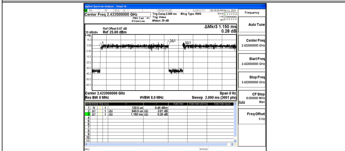
NTNV-11N40MIMO-Ant2-2422
