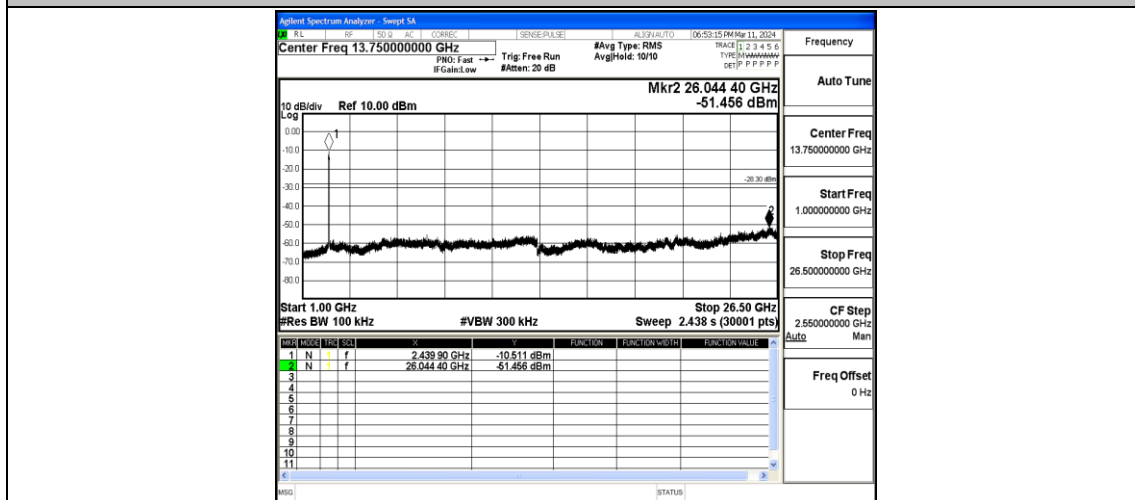
11N40MIMO-Ant2-2437-1000~26500-PASS
