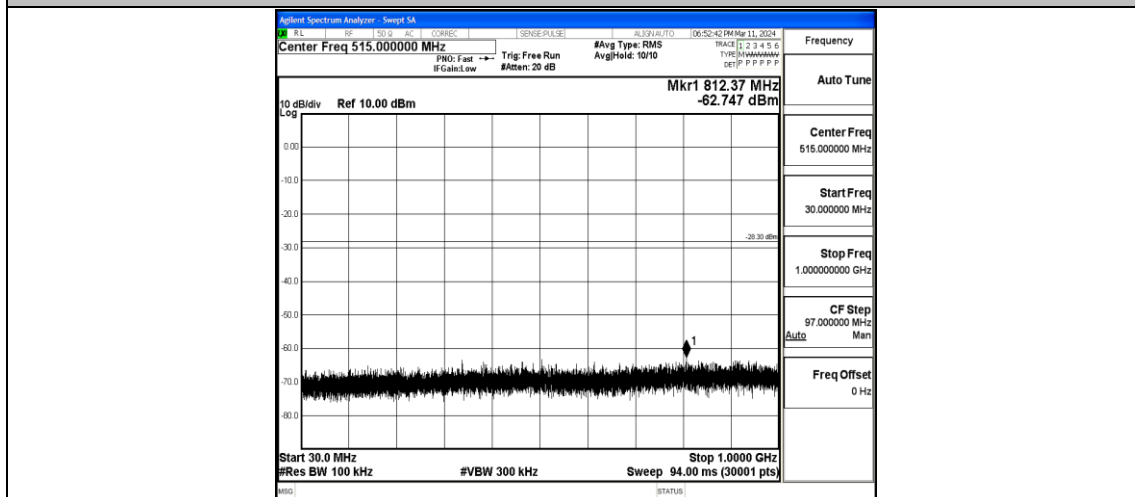
11N40MIMO-Ant2-2437-30~1000-PASS
