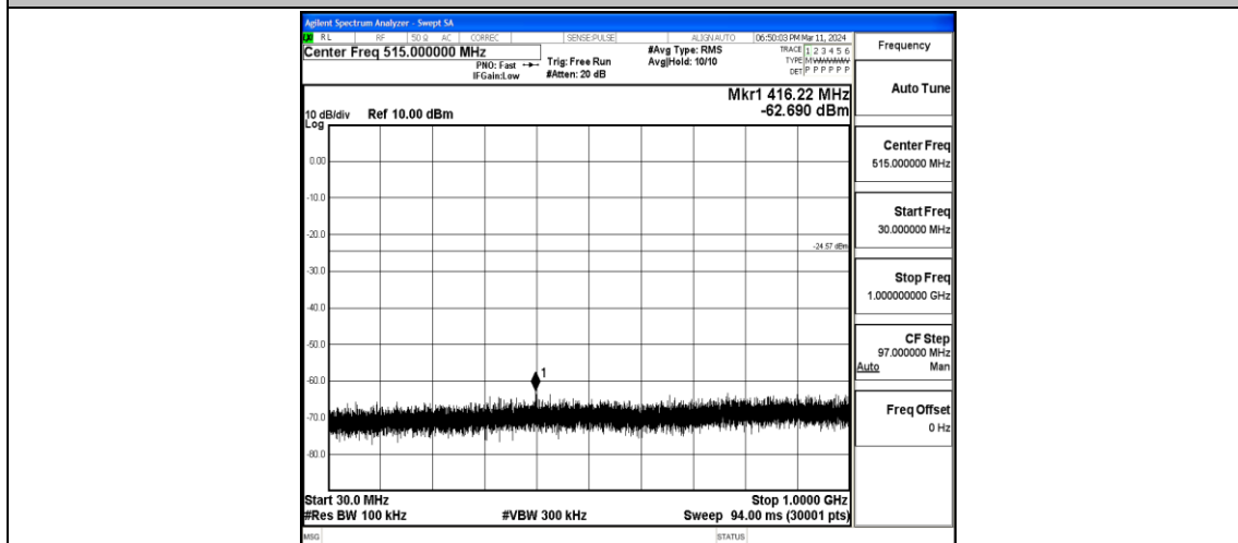
11N40MIMO-Ant1-2437-30~1000-PASS
