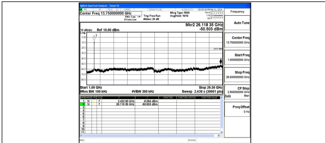
11N40MIMO-Ant1-2437-1000~26500-PASS
