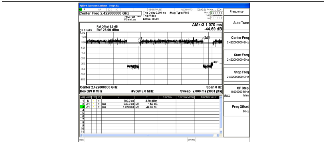
NTNV-11N40MIMO-Ant1-2422
