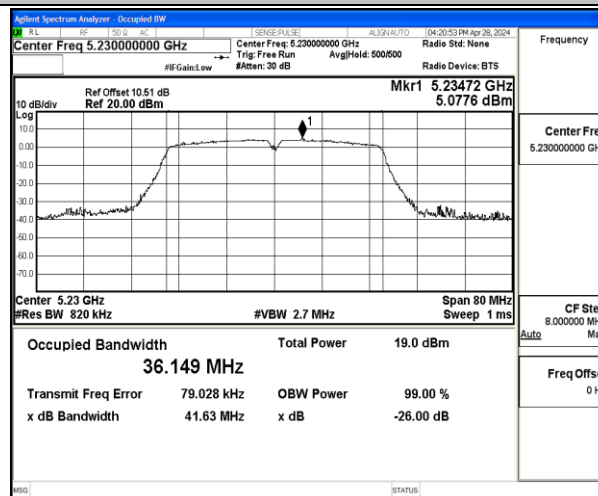
11AC40MIMO-Ant2-5230
