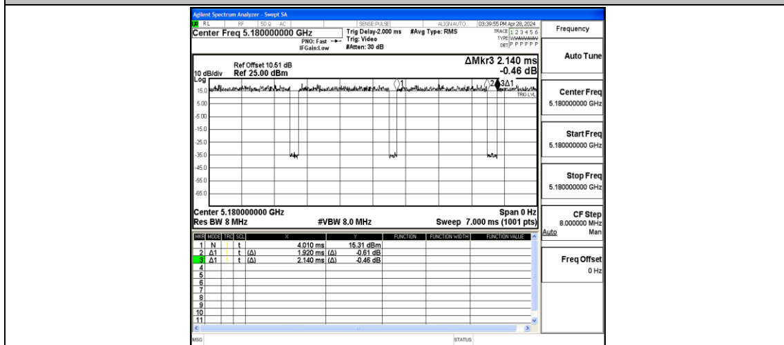
NTNV-11N20MIMO-Ant2-5180
