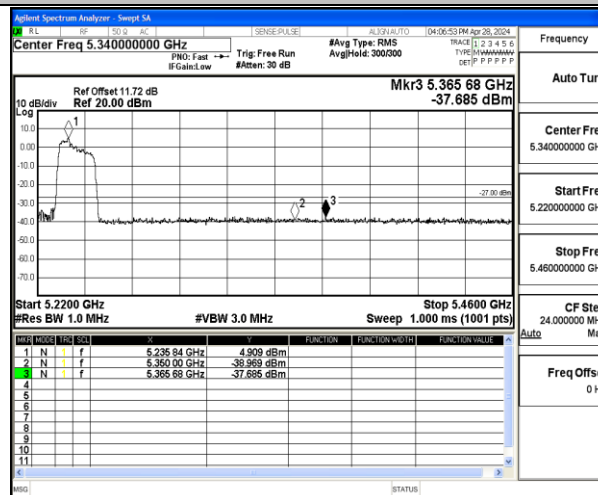
11AC20MIMO-Ant1-5240-PASS
