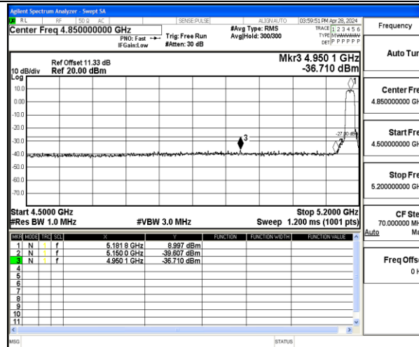
11AC20MIMO-Ant1-5180-PASS
