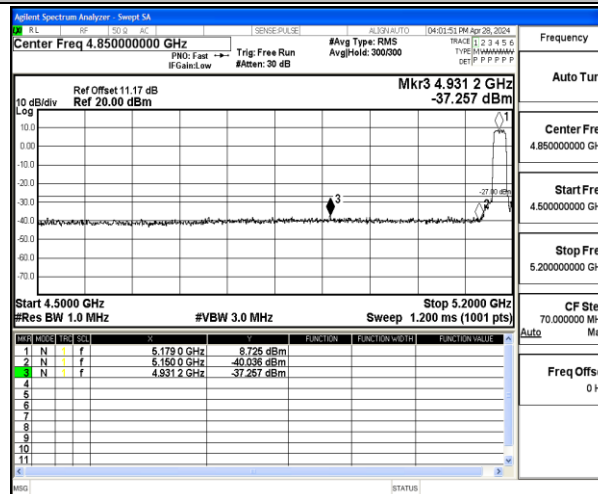
11AC20MIMO-Ant2-5180-PASS
