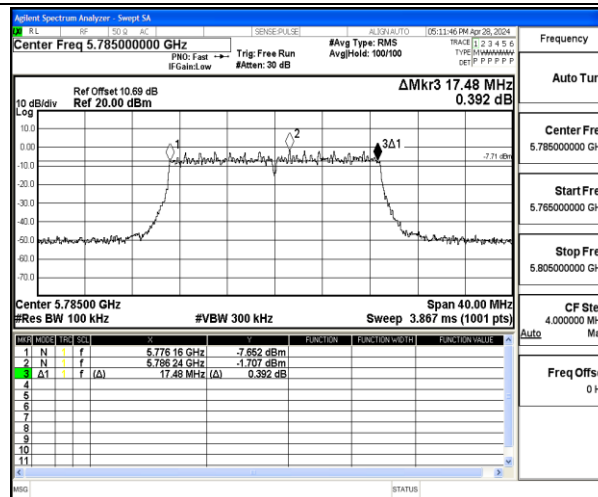
11AC20MIMO-Ant1-5785-PASS
