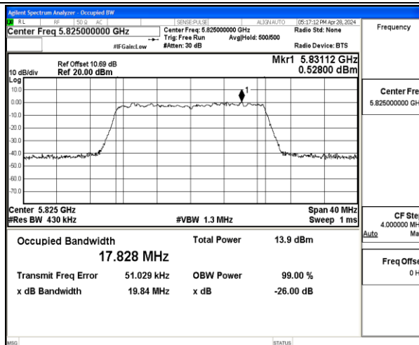
11AC20MIMO-Ant2-5825
