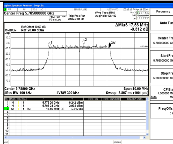
11AC20MIMO-Ant2-5785-PASS
