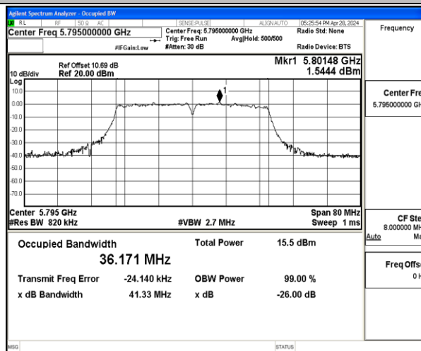
11AC40MIMO-Ant2-5795
