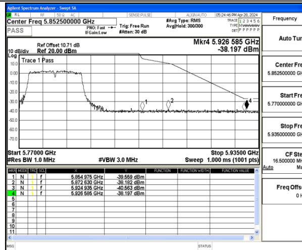
11AC40MIMO-Ant1-5795-PASS
