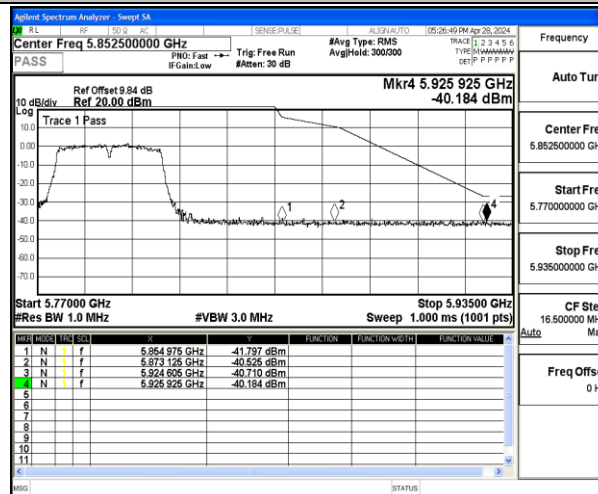
11AC40MIMO-Ant2-5795-PASS
