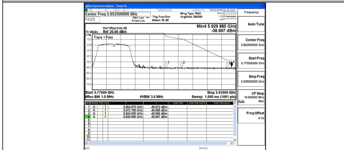
11N40MIMO-Ant2-5795-PASS
