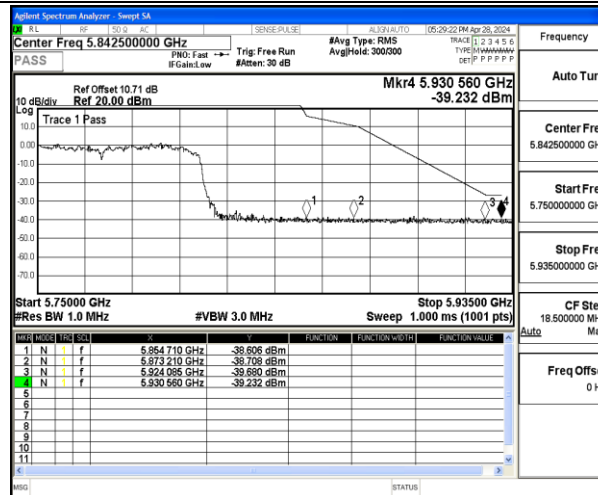
11AC80MIMO-Ant1-5775-PASS
