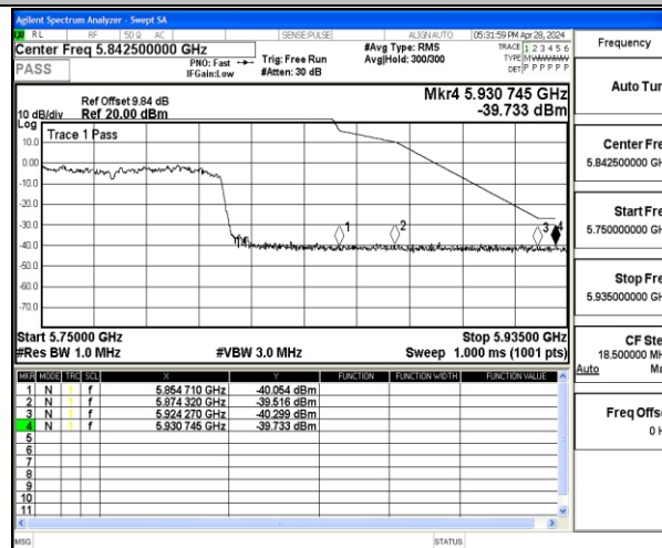
11AC80MIMO-Ant2-5775-PASS
