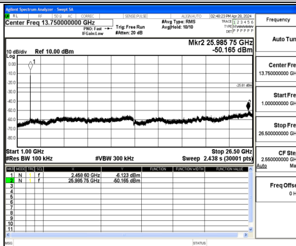
11G-Ant2-2462-1000~26500-PASS
