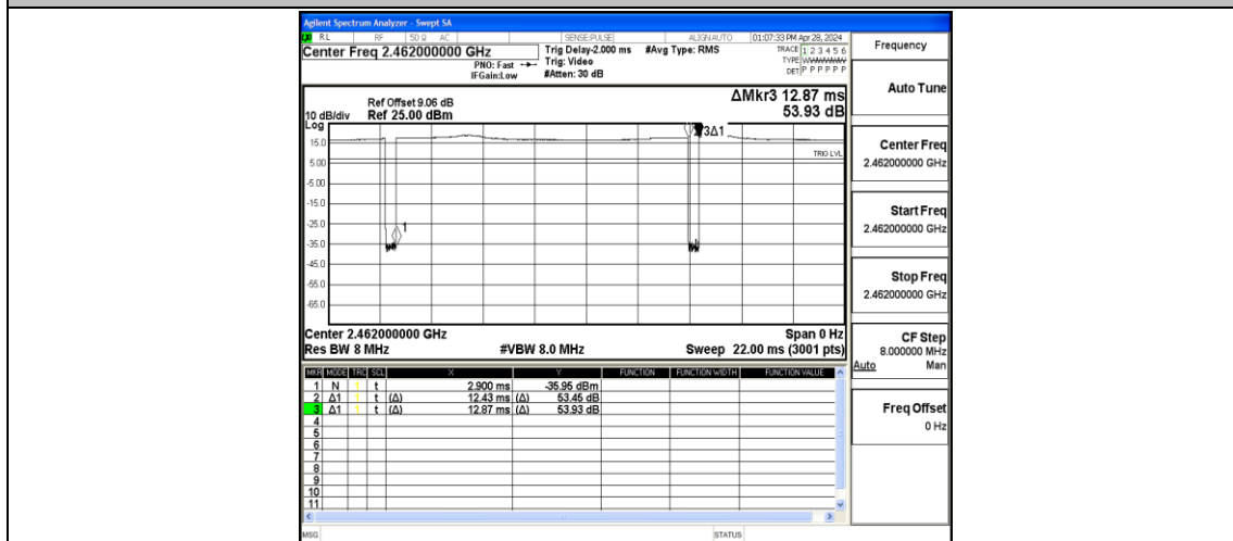
NTNV-11B-Ant1-2462
