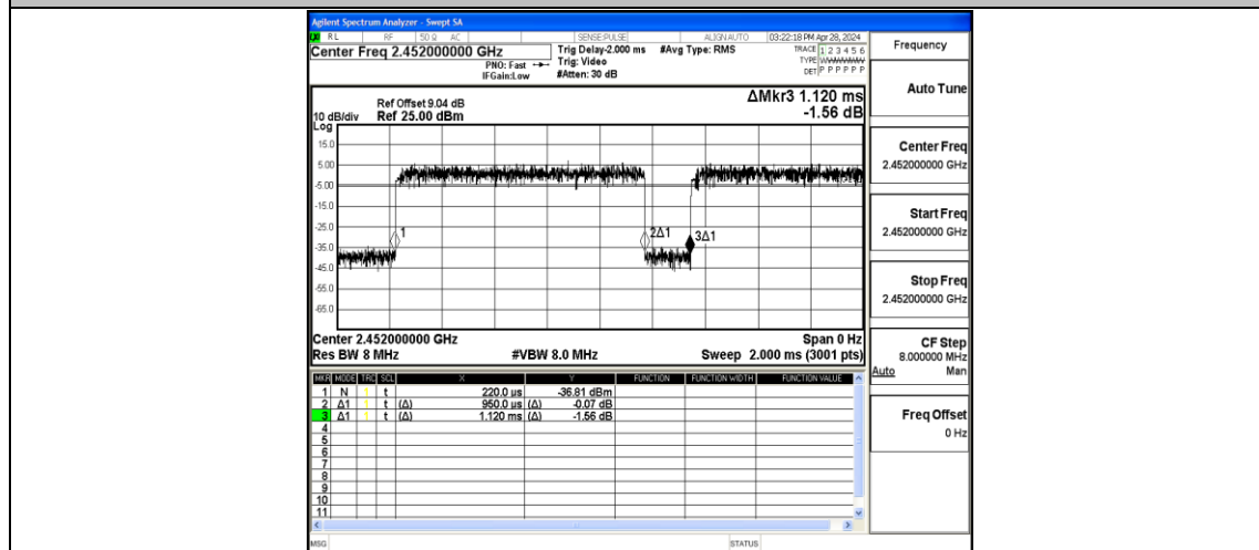
NTNV-11N40MIMO-Ant2-2452
