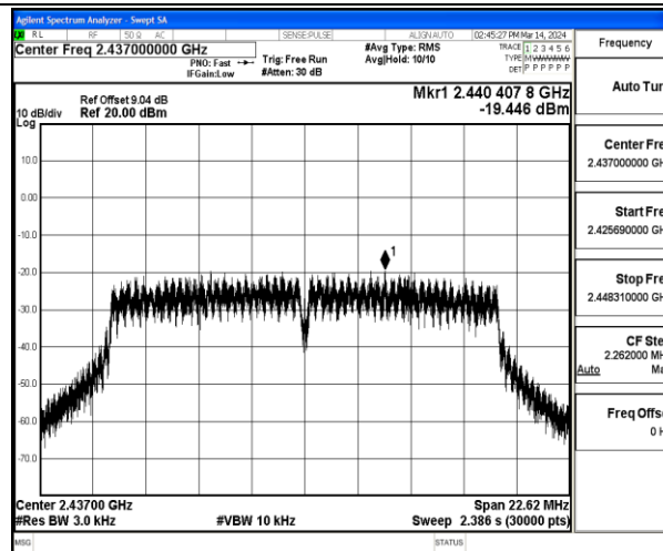
11G-Ant2-2437-PASS
