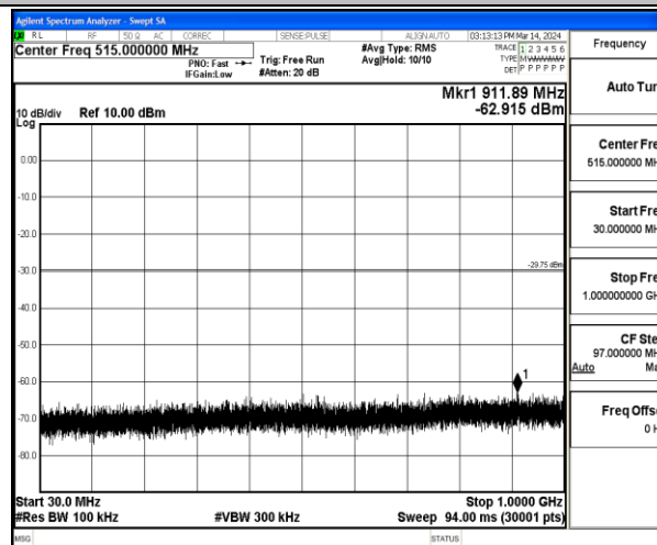
11N40MIMO-Ant2-2422-30~1000-PASS
