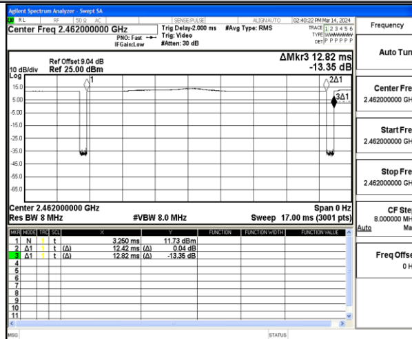
NTNV-11B-Ant2-2462
