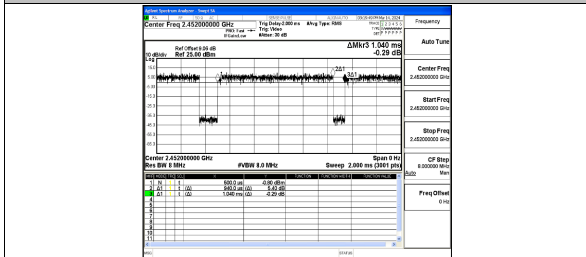
NTNV-11N40MIMO-Ant1-2452
