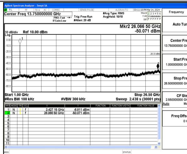
11N40MIMO-Ant1-2422-1000~26500-PASS
