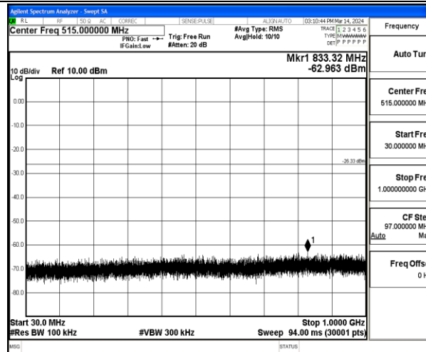
11N40MIMO-Ant1-2422-30~1000-PASS
