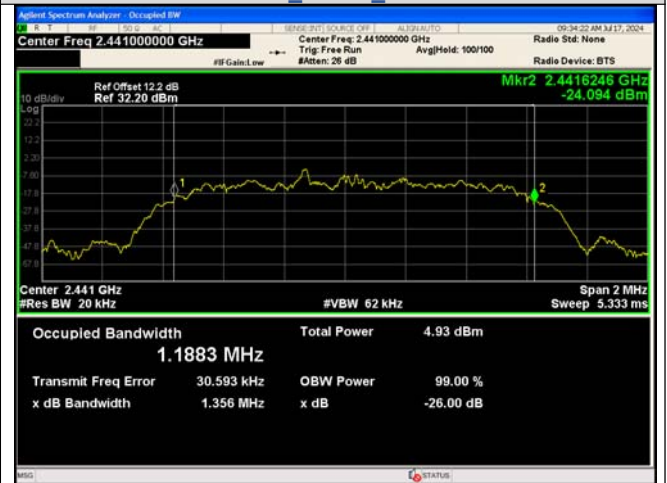
\pi/4 DQPSK_2-DH5_Channel 39
