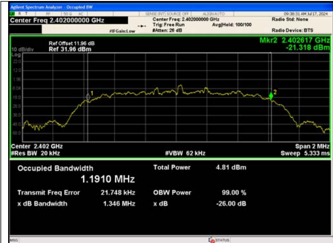
8DPSK_3-DH5_Channel 0
