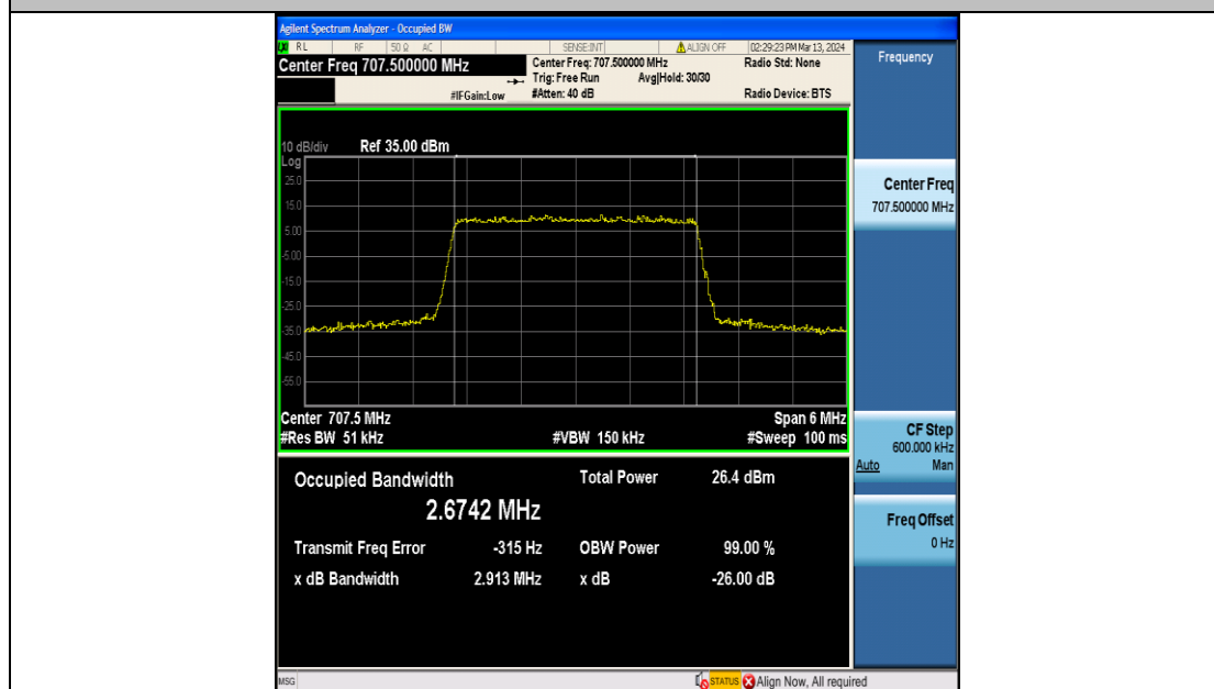
Band12-3MHz-16QAM-23095-15RB#0-PASS
