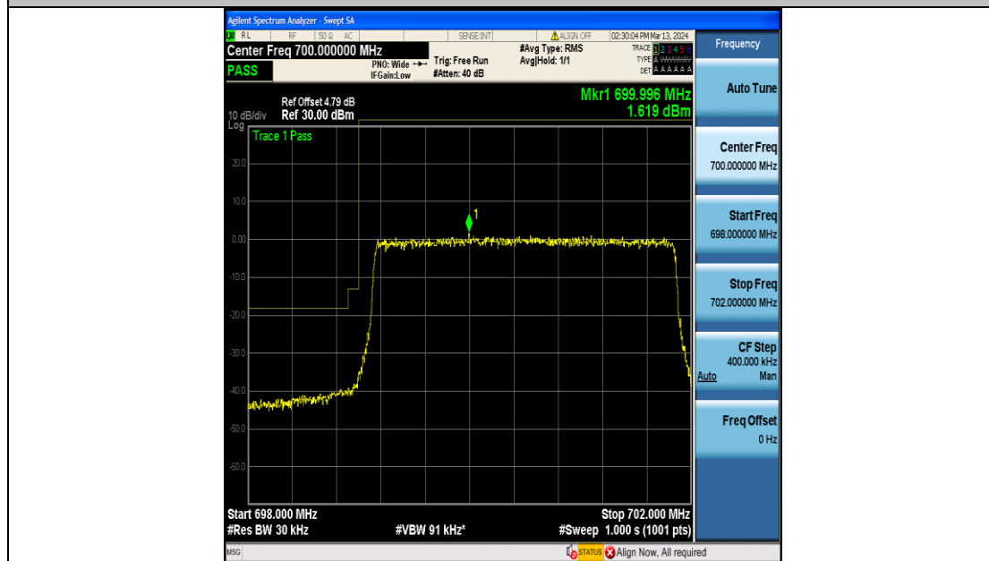
Band12_3MHz_QPSK_23025_15RB#0
