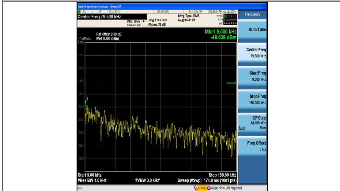
Band12_1.4MHz_16QAM_23173_6RB#0_0.009~0.15_0.009~0.15
