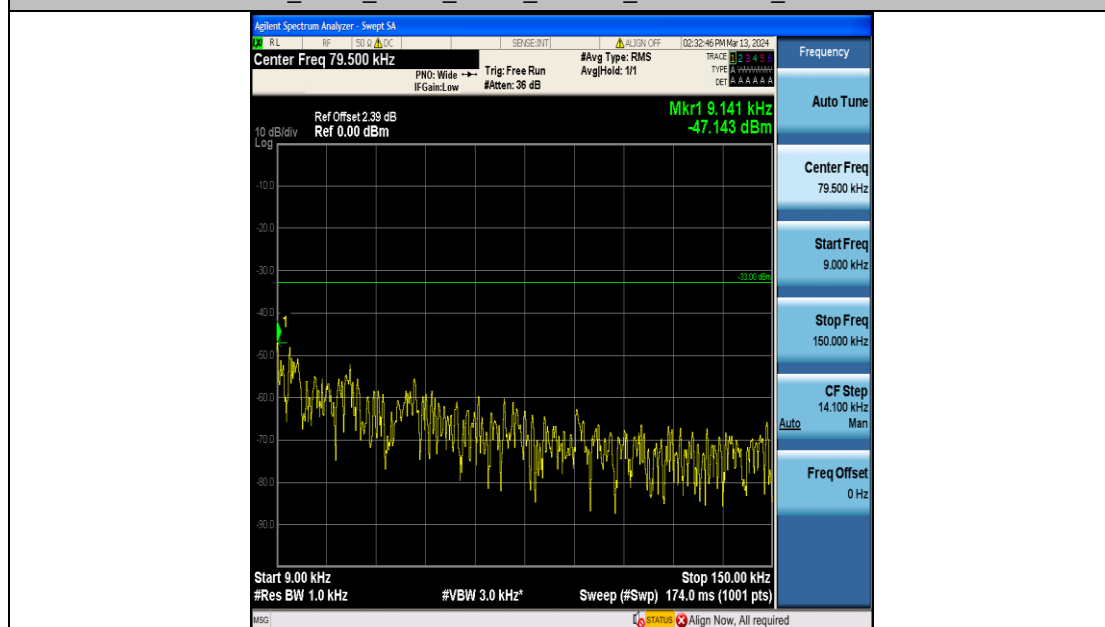
Band12_3MHz_16QAM_23095_15RB#0_0.009~0.15_0.009~0.15
