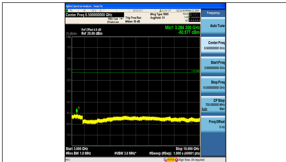
Band12_3MHz_QPSK_23095_15RB#0_3000~10000_3000~10000
