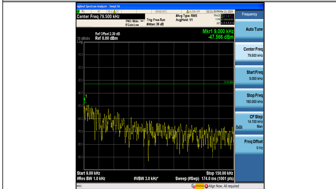
Band12_1.4MHz_16QAM_23095_6RB#0_0.009~0.15_0.009~0.15
