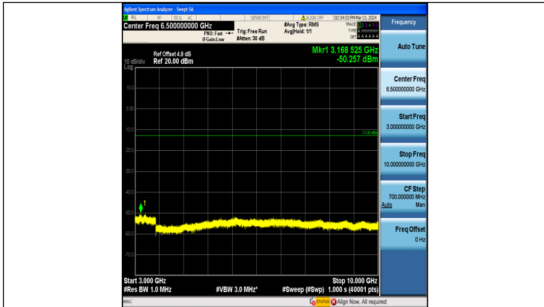
Band12_3MHz_QPSK_23165_15RB#0_3000~10000_3000~10000
