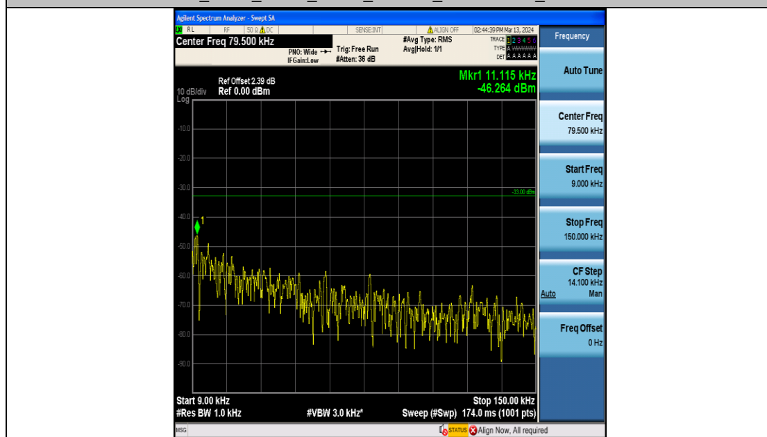
Band12_5MHz_16QAM_23095_25RB#0_0.009~0.15_0.009~0.15
