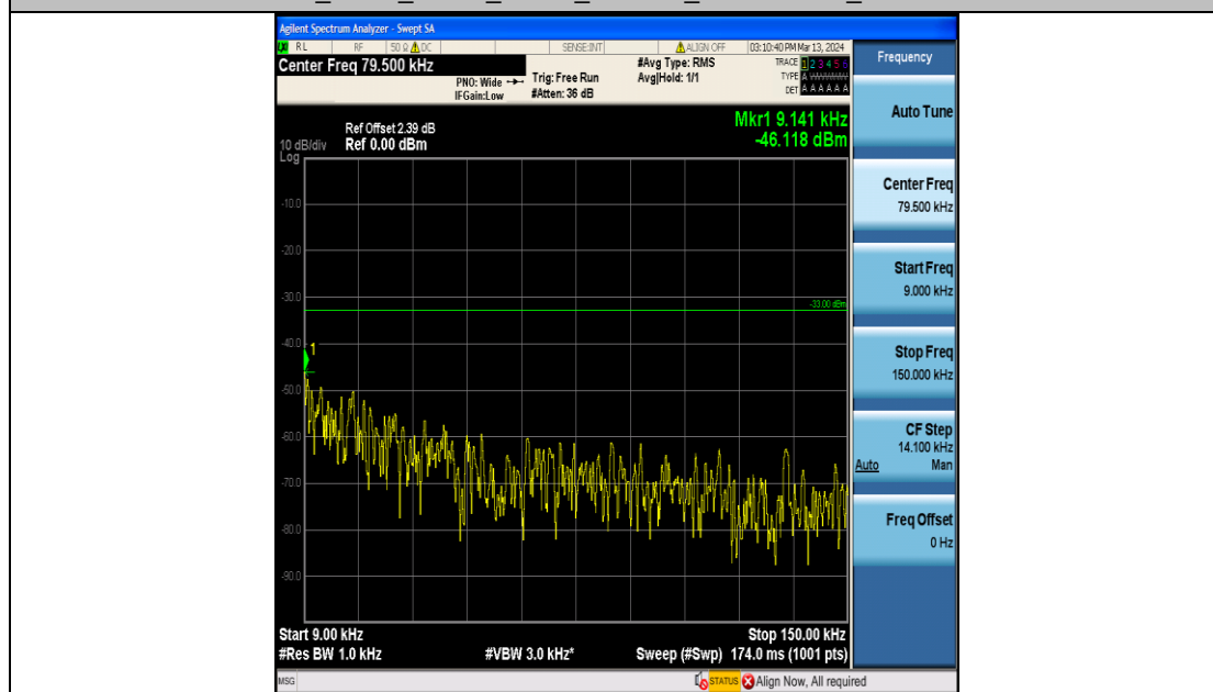
Band13_5MHz_16QAM_23230_25RB#0_0.009~0.15_0.009~0.15
