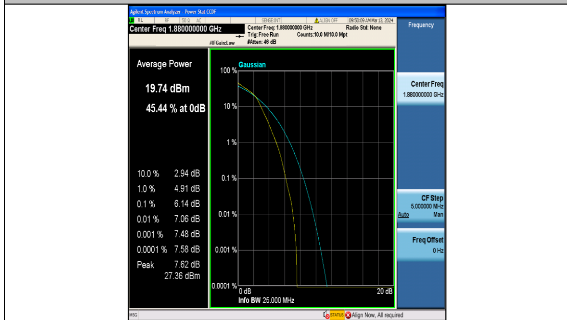
Band2-1.4MHz-16QAM-18900-6RB#0-PASS
