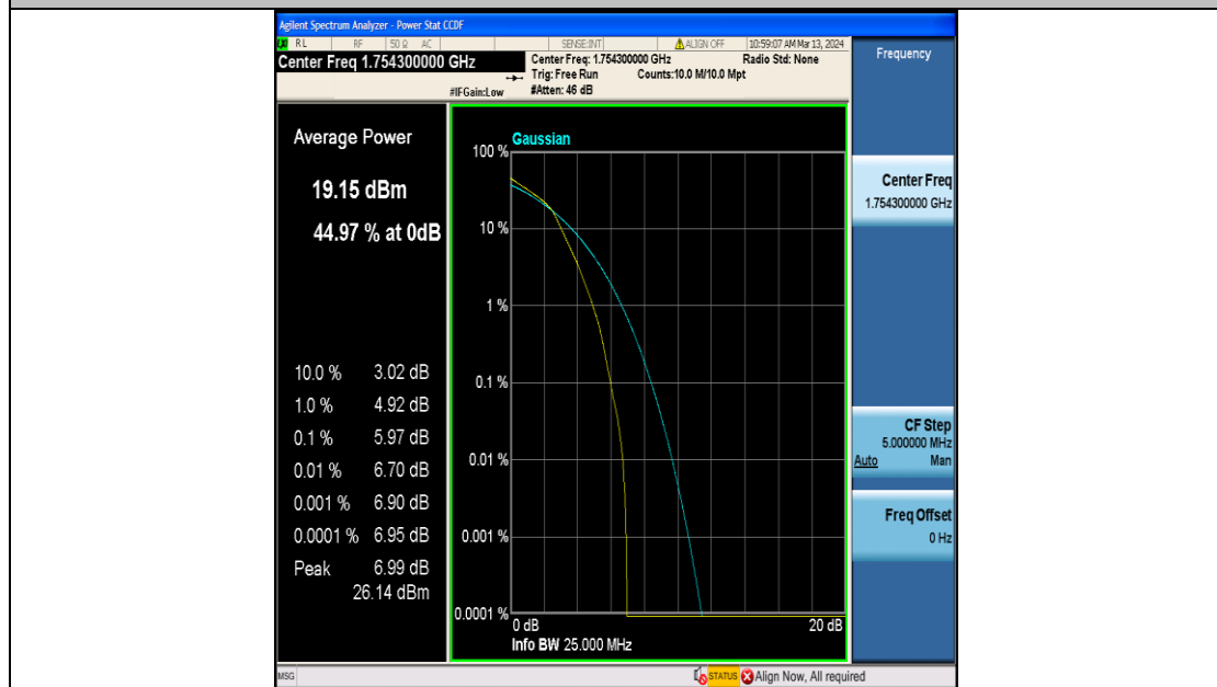
Band4-1.4MHz-16QAM-20393-6RB#0-PASS
