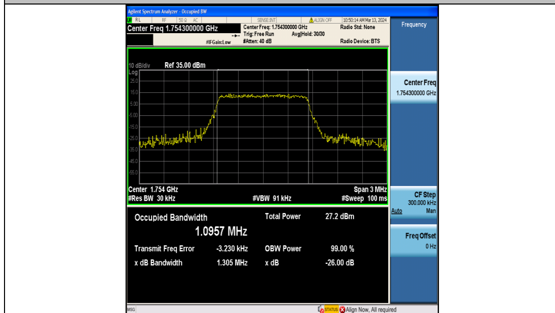
Band4-1.4MHz-16QAM-20393-6RB#0-PASS
