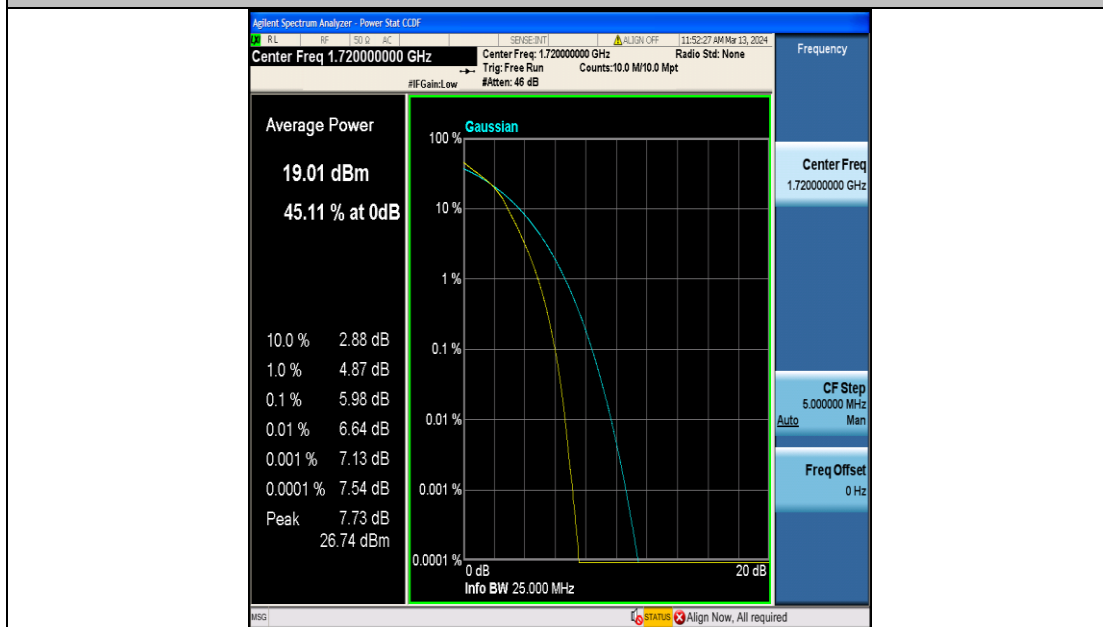
Band4-20MHz-16QAM-20050-100RB#0-PASS
