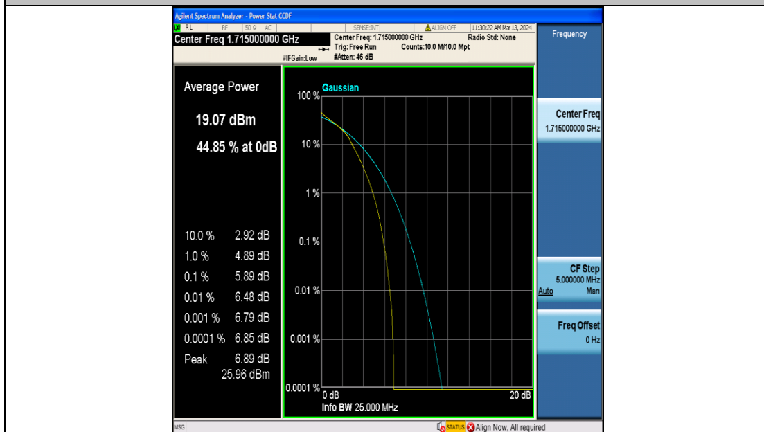
Band4-10MHz-16QAM-20000-50RB#0-PASS
