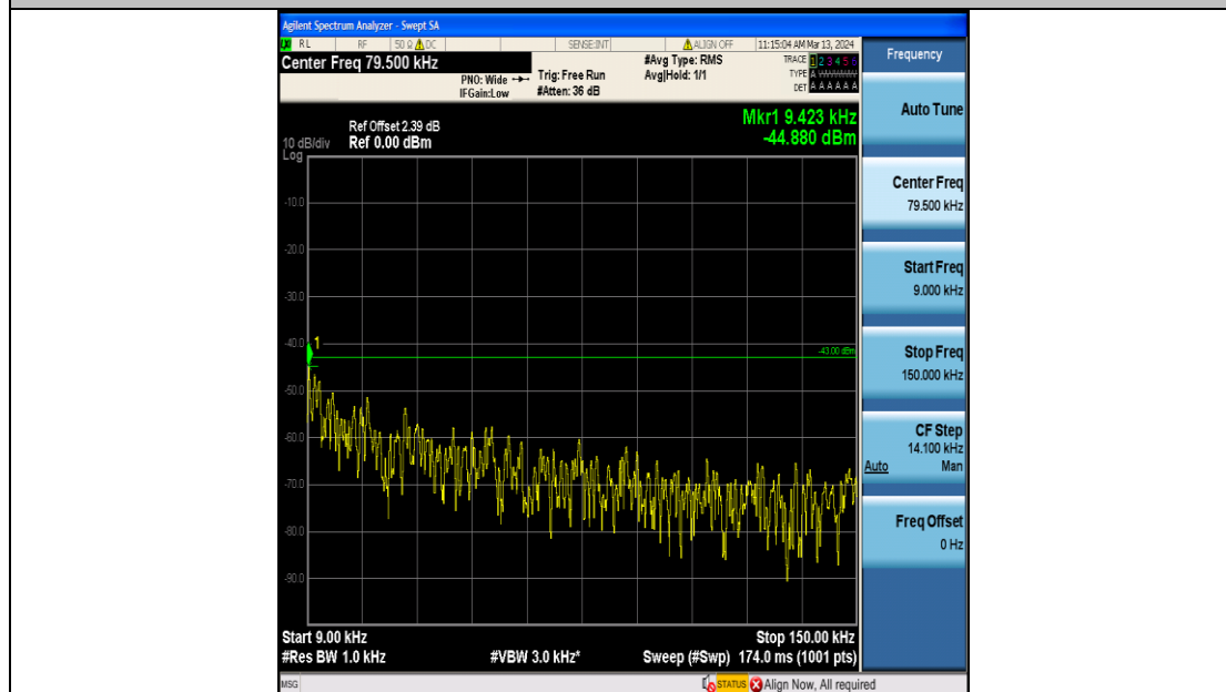
Band4_5MHz_QPSK_20375_25RB#0_0.009~0.15_0.009~0.15
