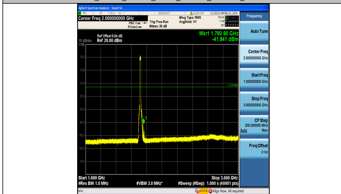
Band4_15MHz_16QAM_20025_75RB#0_1000~3000_1000~3000
