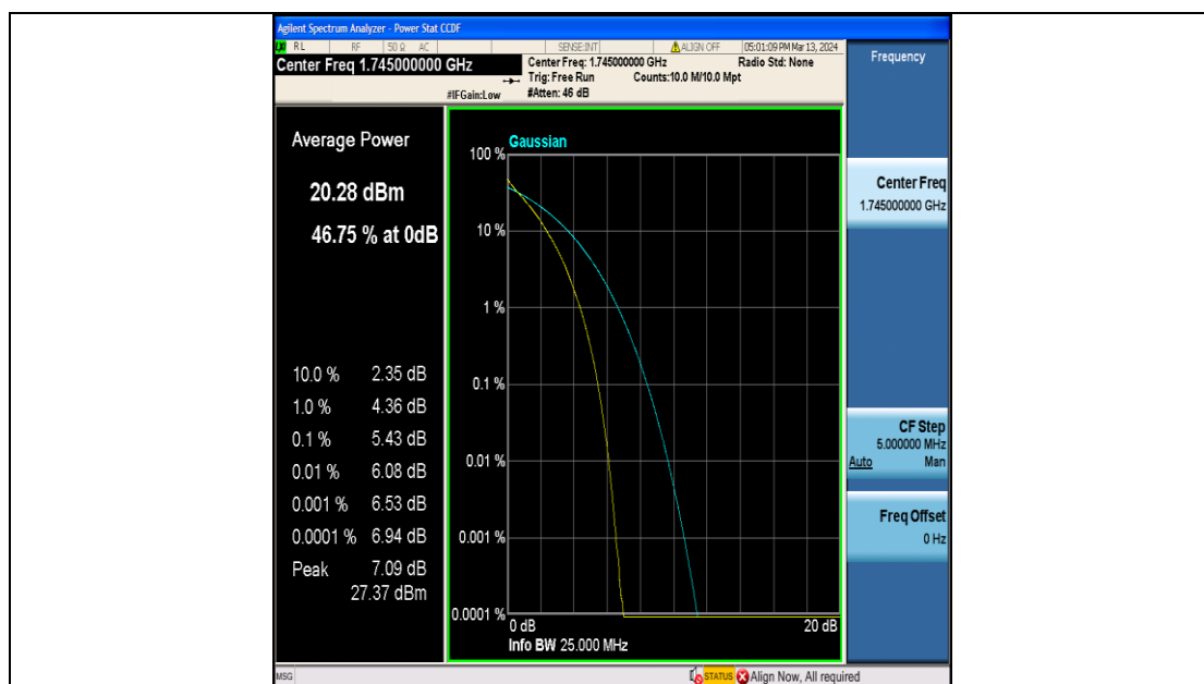
Band66-20MHz-QPSK-132322-100RB#0-PASS
