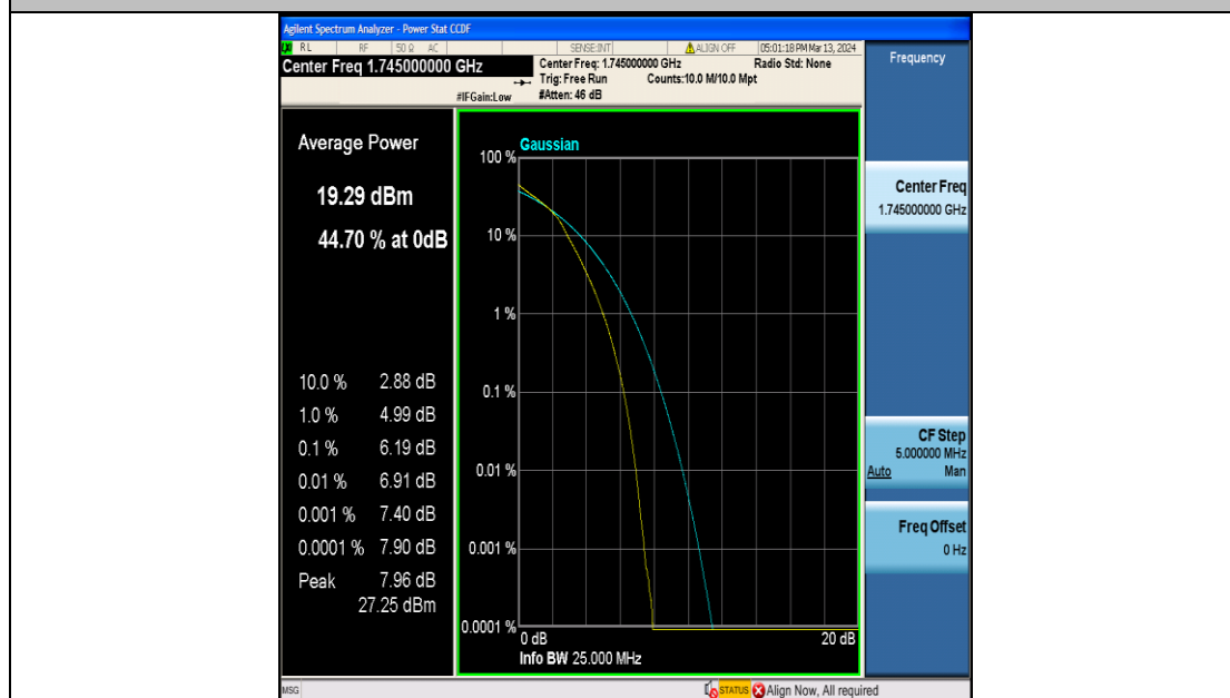
Band66-20MHz-16QAM-132322-100RB#0-PASS
