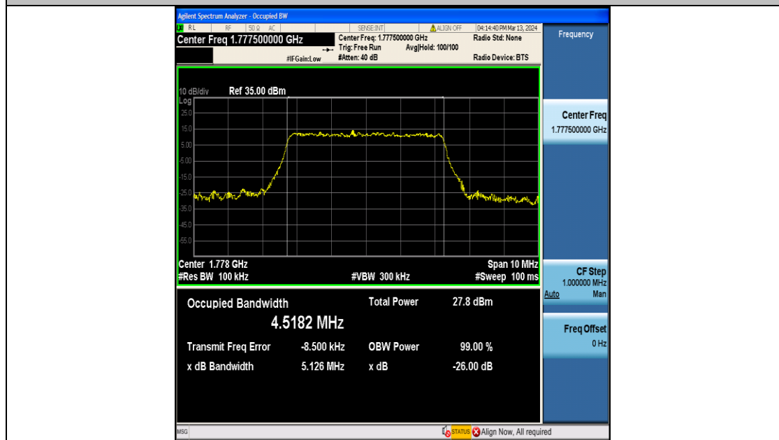
Band66-5MHz-16QAM-132647-25RB#0-PASS
