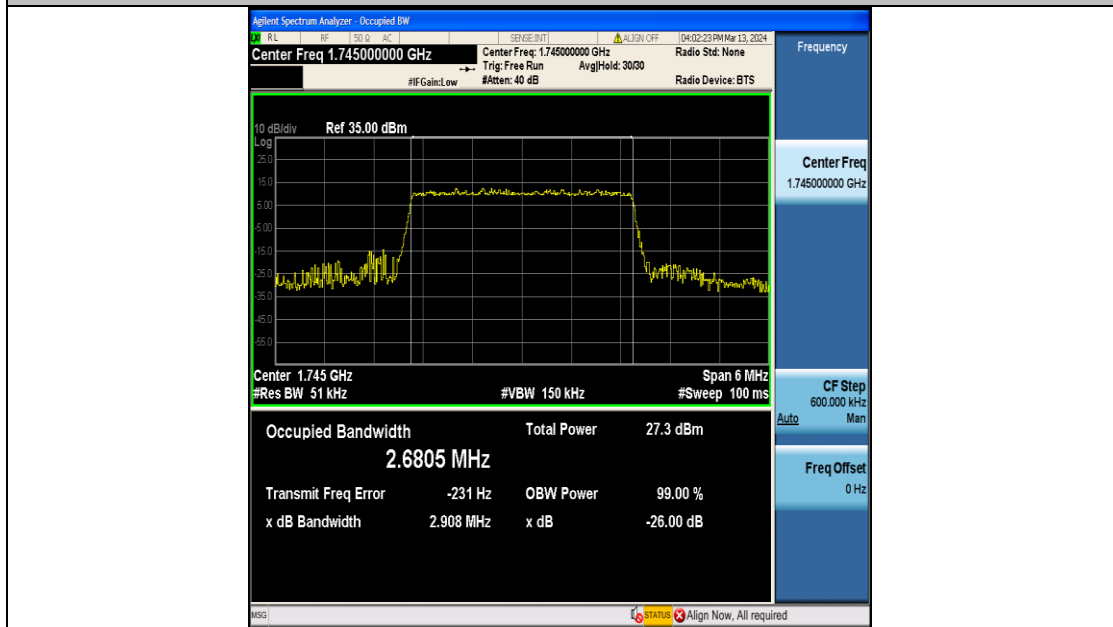
Band66-3MHz-16QAM-132322-15RB#0-PASS
