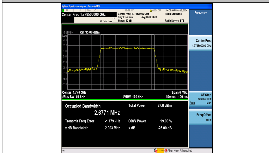
Band66-3MHz-16QAM-132657-15RB#0-PASS
