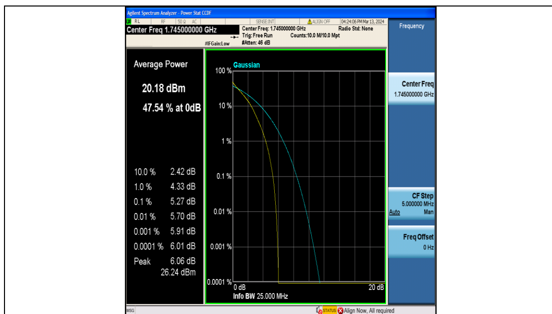
Band66-5MHz-QPSK-132322-25RB#0-PASS
