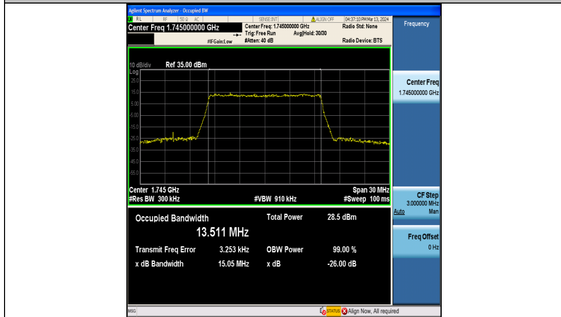
Band66-15MHz-16QAM-132322-75RB#0-PASS
