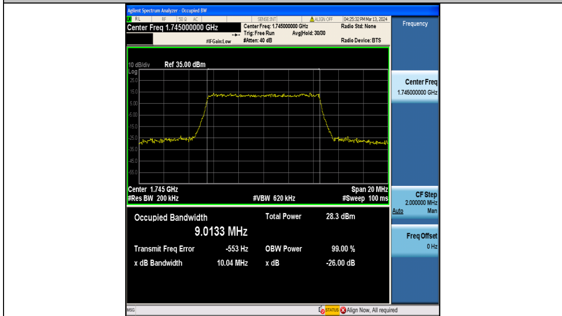
Band66-10MHz-16QAM-132322-50RB#0-PASS
