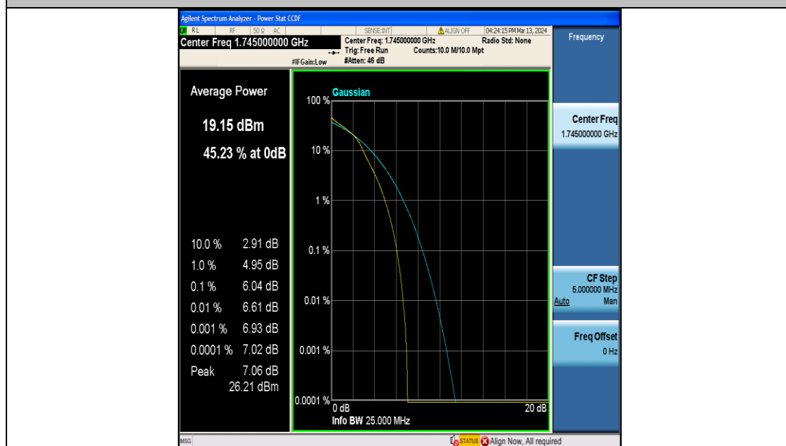
Band66-5MHz-16QAM-132322-25RB#0-PASS
