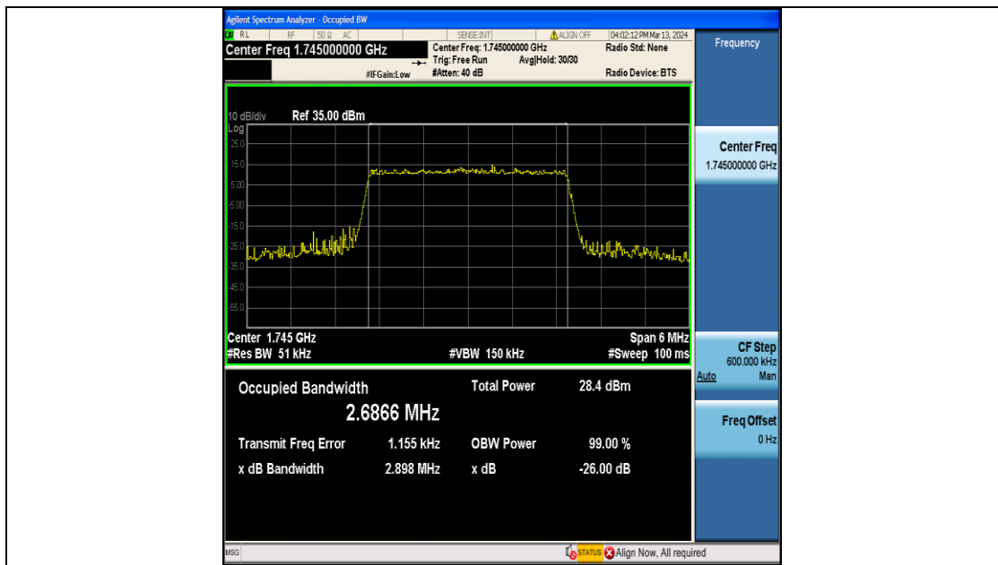
Band66-3MHz-QPSK-132322-15RB#0-PASS
