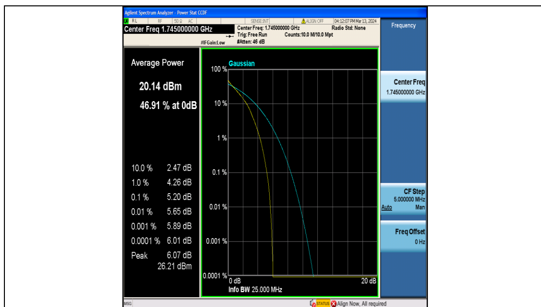
Band66-3MHz-QPSK-132322-15RB#0-PASS
