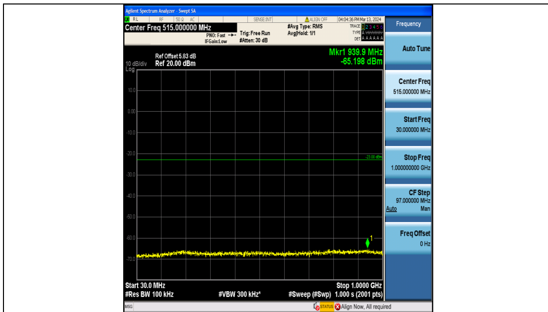
Band66_3MHz_16QAM_131987_15RB#0_30~1000_30~1000
