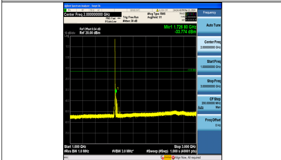
Band66_3MHz_16QAM_131987_15RB#0_1000~3000_1000~3000
