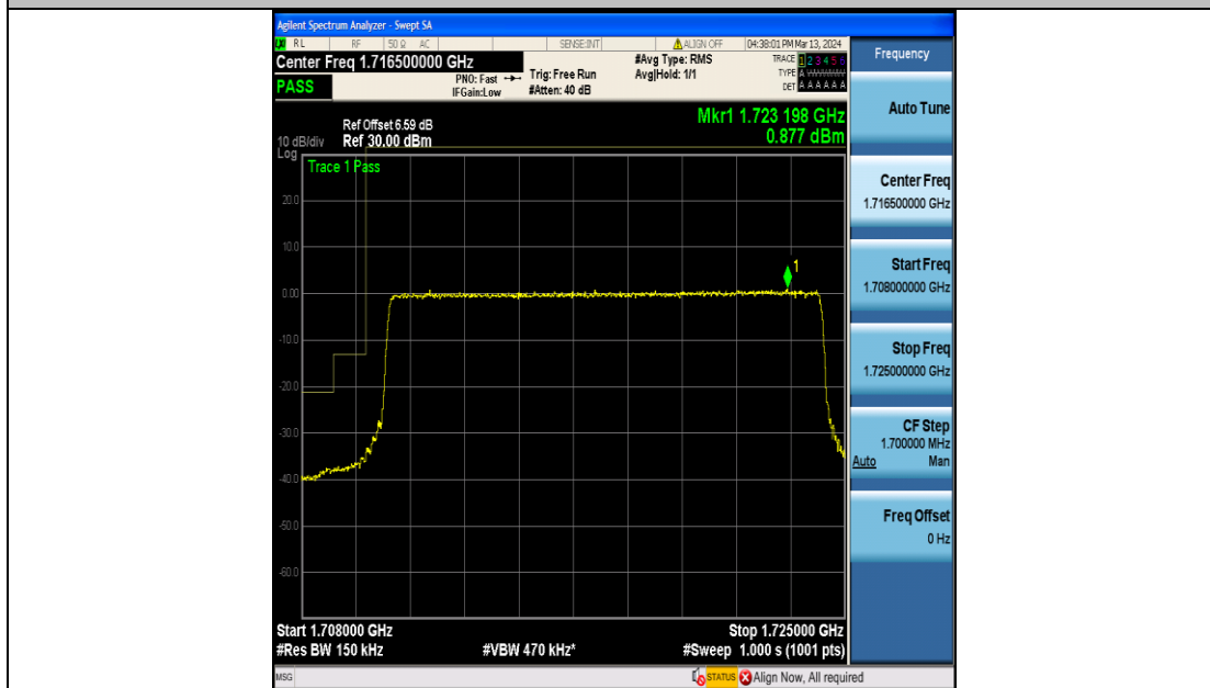
Band66_15MHz_16QAM_132047_75RB#0
