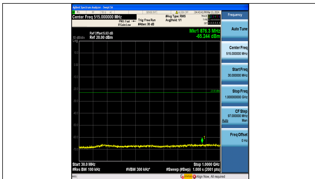
Band66_15MHz_16QAM_132597_75RB#0_30~1000_30~1000
