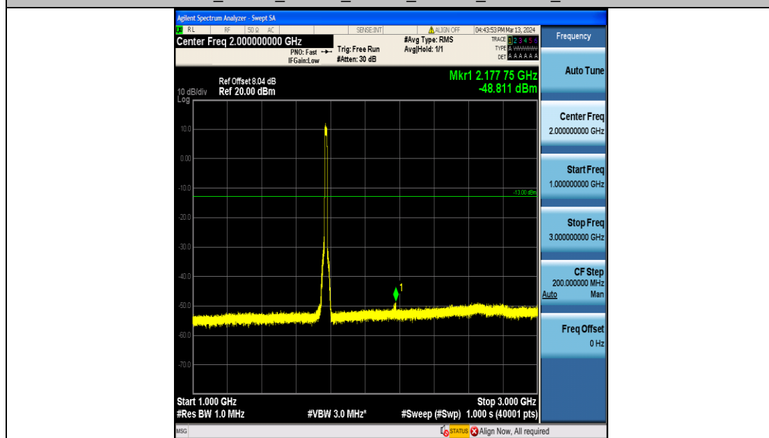
Band66_15MHz_16QAM_132597_75RB#0_1000~3000_1000~3000
