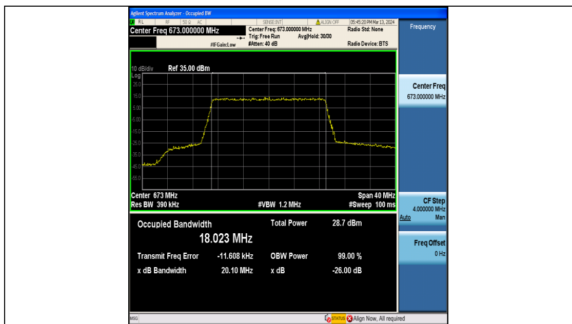
Band71-20MHz-QPSK-133222-100RB#0-PASS
