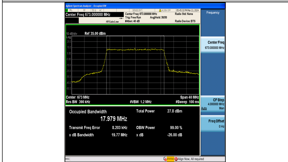
Band71-20MHz-16QAM-133222-100RB#0-PASS
