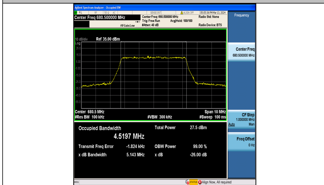
Band71-5MHz-16QAM-133297-25RB#0-PASS
