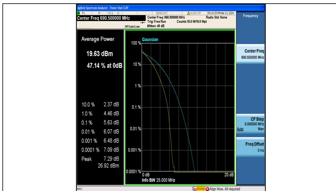
Band71-15MHz-QPSK-133397-75RB#0-PASS
