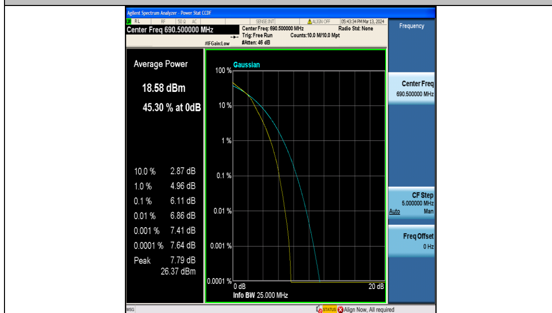
Band71-15MHz-16QAM-133397-75RB#0-PASS
