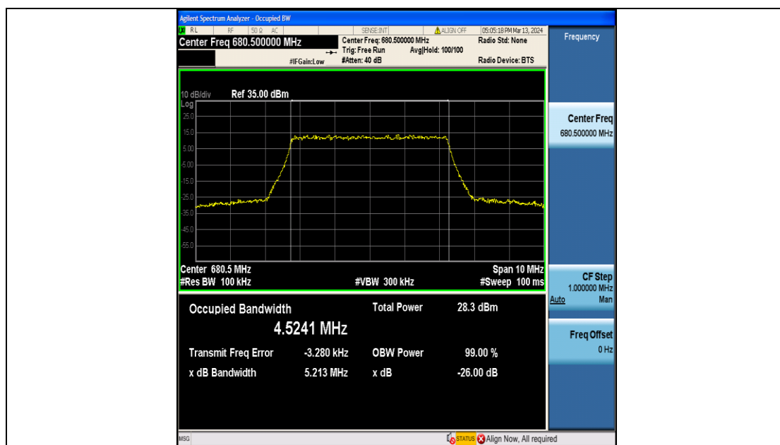
Band71-5MHz-QPSK-133297-25RB#0-PASS
