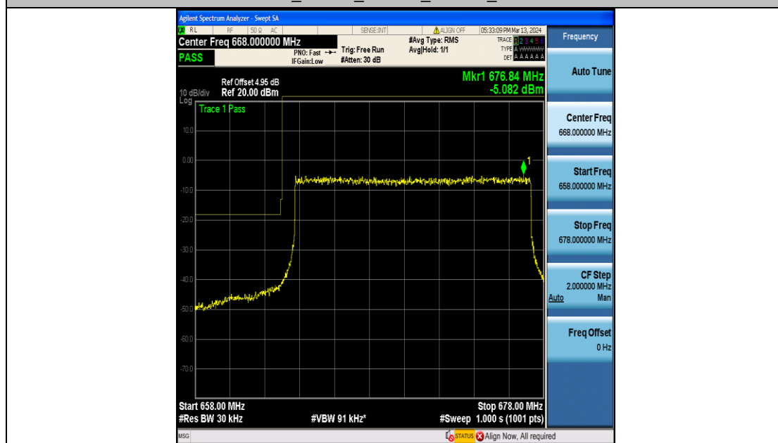
Band71_15MHz_QPSK_133197_75RB#0
