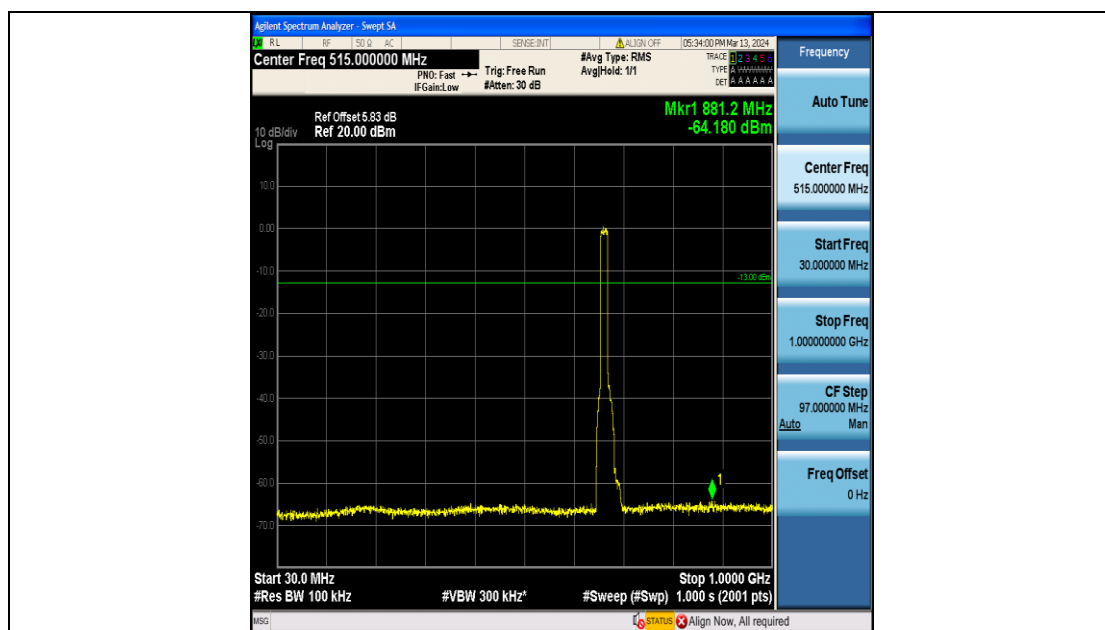
Band71_15MHz_QPSK_133197_75RB#0_30~1000_30~1000
