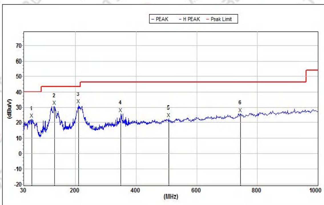
Mode 1 Horizontal
