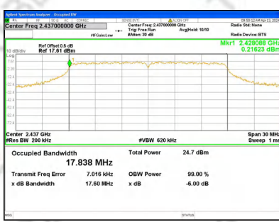
99% Bandwidth Mode8CH 06
