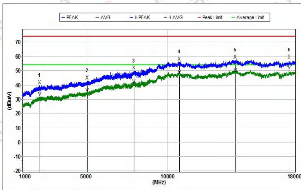
Mode 1 Horizontal
