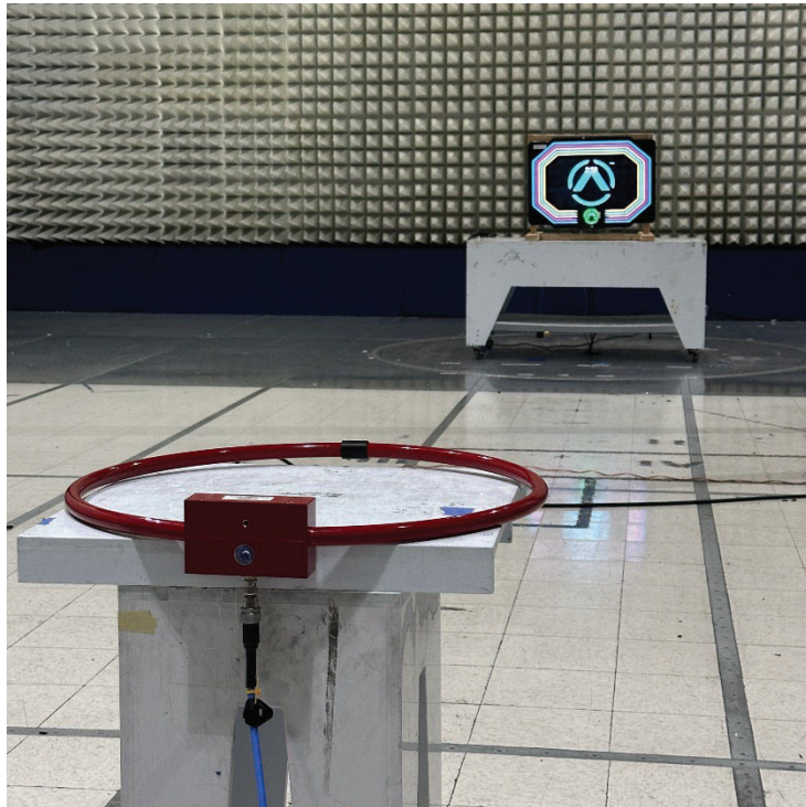
Electromagnetic Radiated Disturbance Setup Photograph
