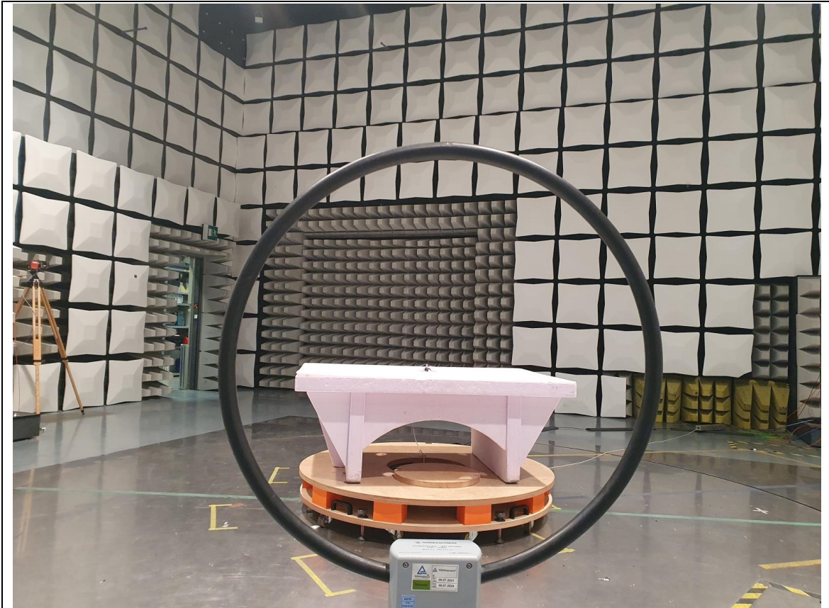
Test Setup: Radiated Measurements (9 kHz - 30 MHz) Parallel polarization Antenna Side
