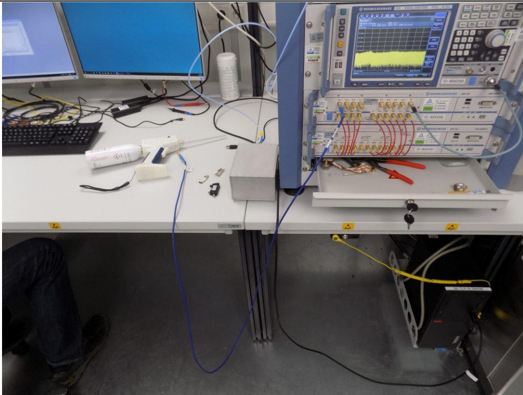
Test setup: Conducted measurements EUT-side
