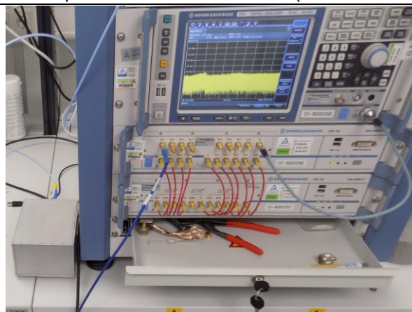
Test Setup: Conducted Measurements T8997 side
