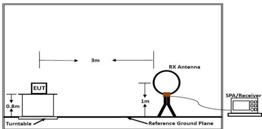
Below 30MHz
