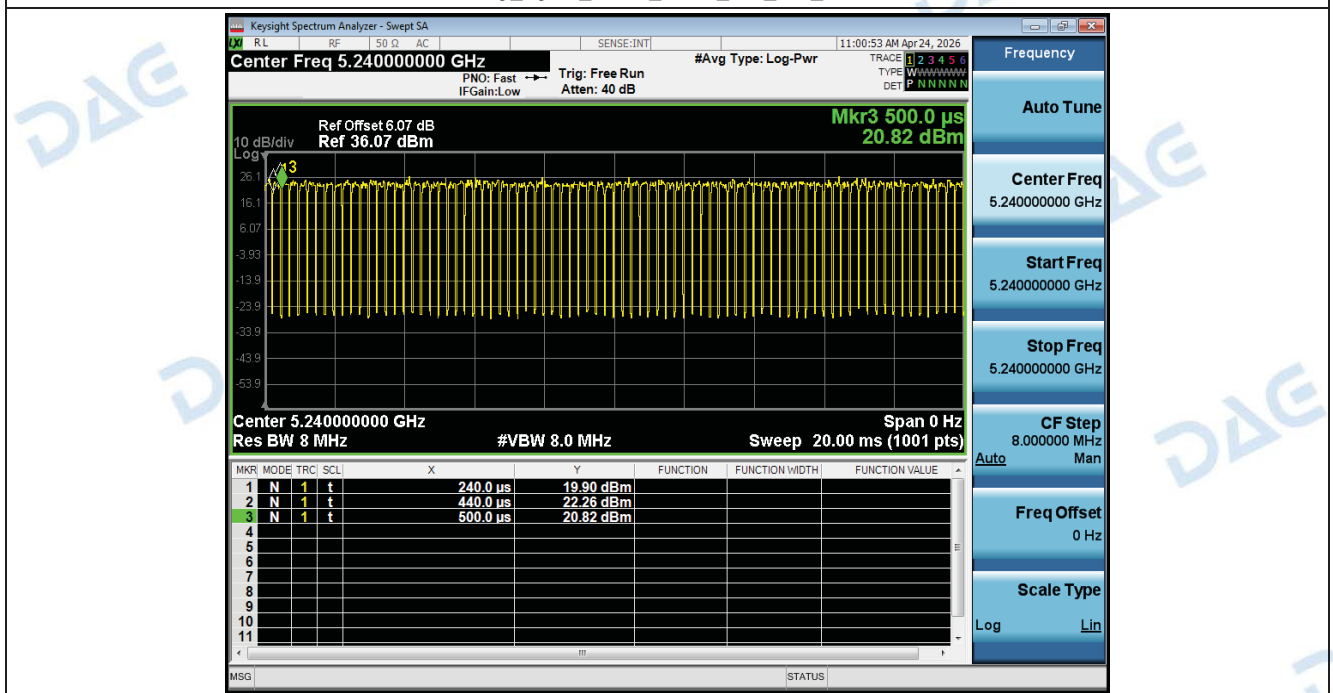
Duty_Cycle_NVNT_ANT1_802_11a_5240
