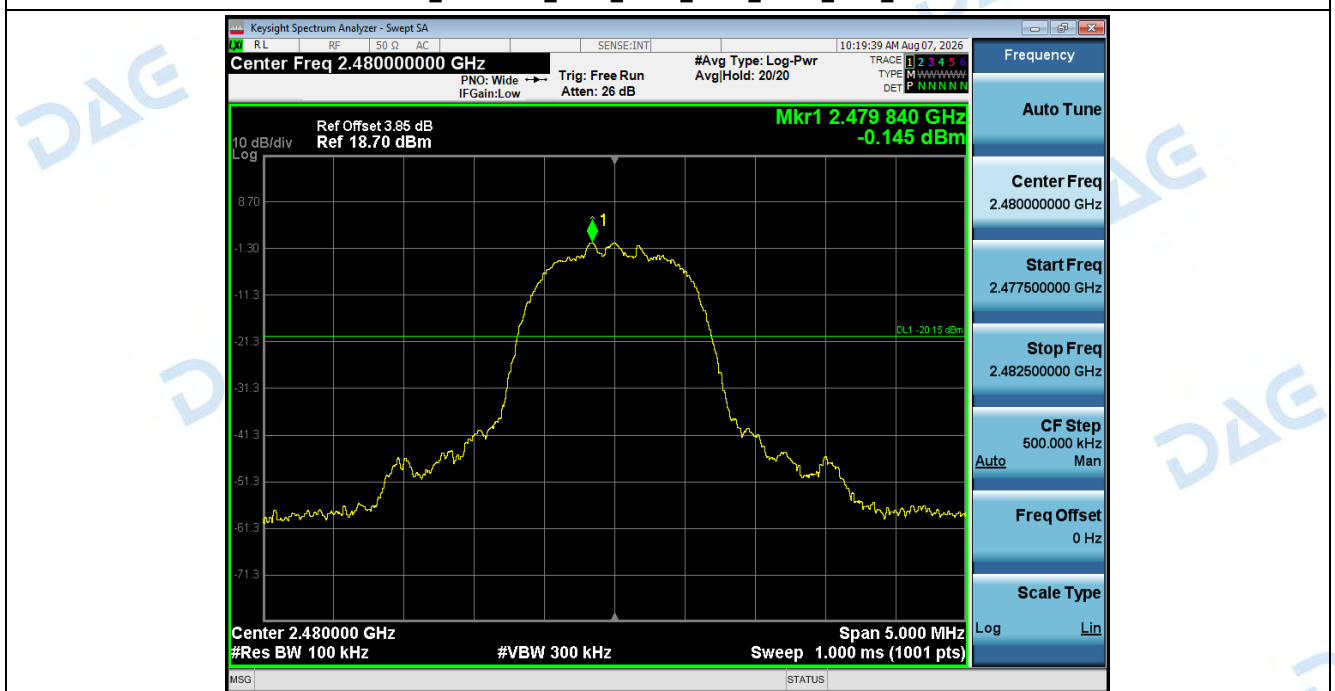
2_Bandedge_NVNT_ANT1_3-DH5_2480_00
