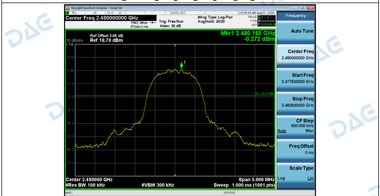
2_Spurious_Emissions_NVNT_ANT1_2-DH5_2480_00
