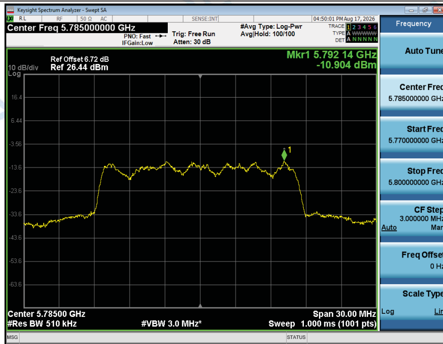
Power_Spectral_Density_NVNT_ANT2_802_11a_5785
