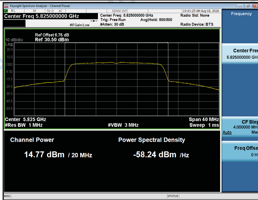
Maximum_Conducted_Output_Power_NVNT_ANT2_802_11n(HT20)_5825
