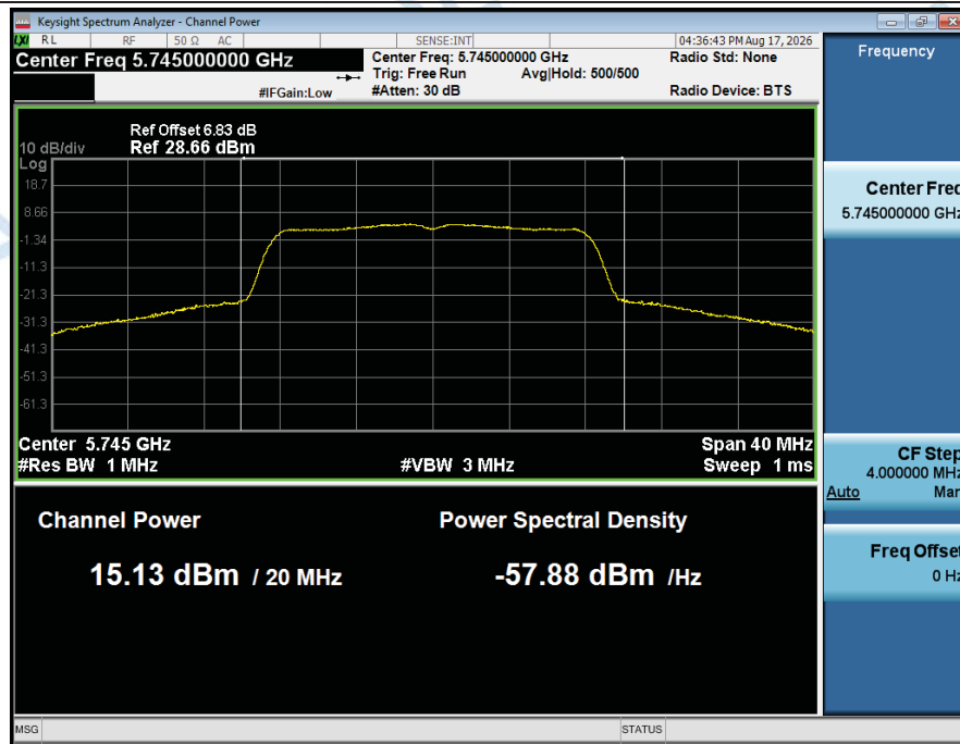
Maximum_Conducted_Output_Power_NVNT_ANT2_802_11a_5745
