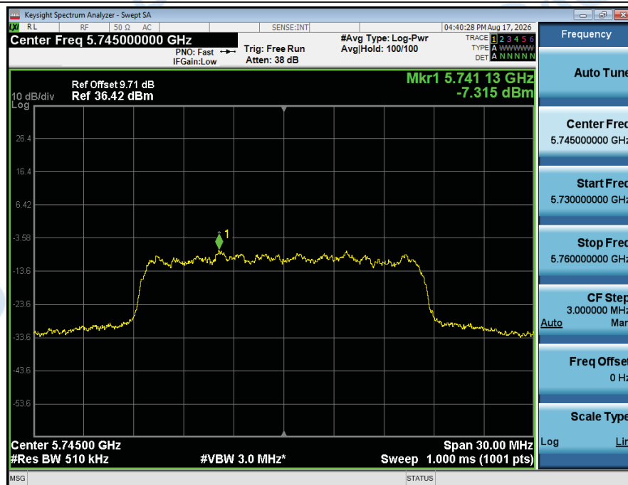
Power_Spectral_Density_NVNT_ANT2_802_11a_5745
