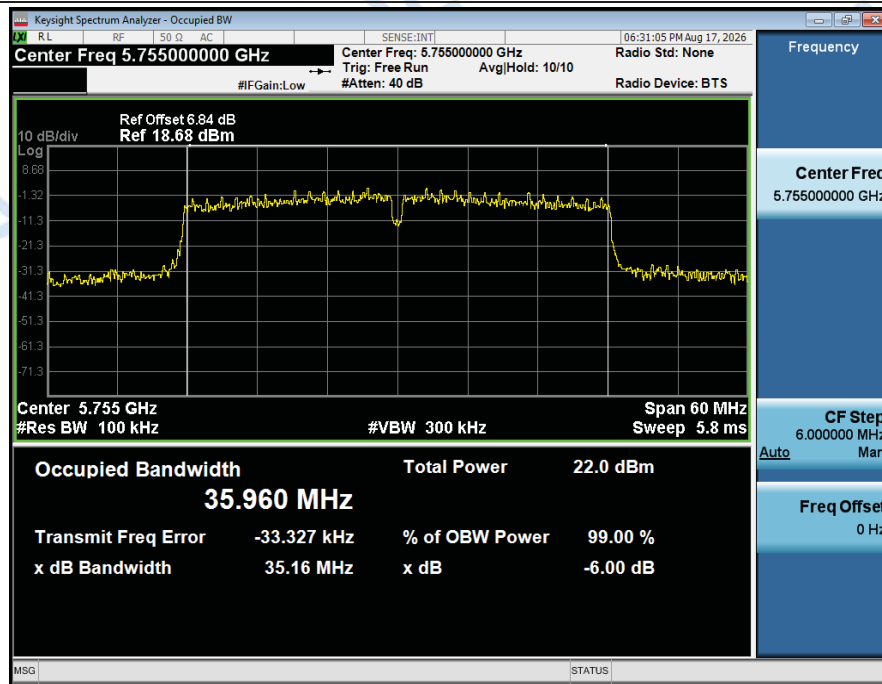
-6dB_Emission_Bandwidth_NVNT_ANT2_802_11n(HT40)_5755_40M
