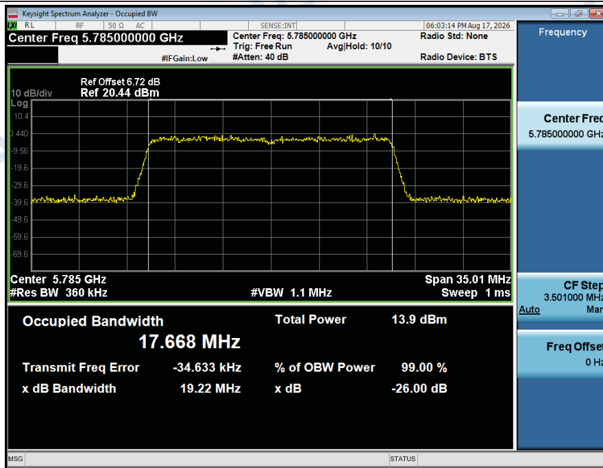
-26BW_NVNT_ANT1_802_11ac(VHT20)_5785
