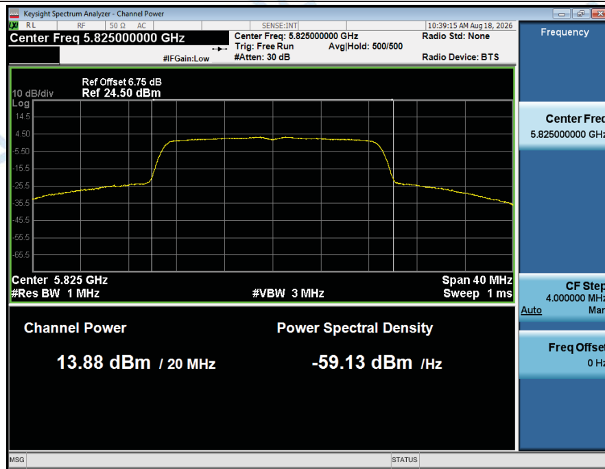
Maximum_Conducted_Output_Power_NVNT_ANT2_802_11ac(VHT20)_5825
