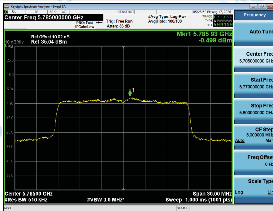
Power_Spectral_Density_NVNT_ANT2_802_11n(HT20)_5785
