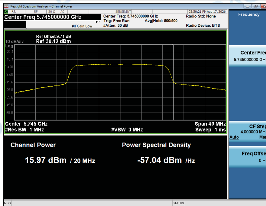
Maximum_Conducted_Output_Power_NVNT_ANT2_802_11n(HT20)_5745
