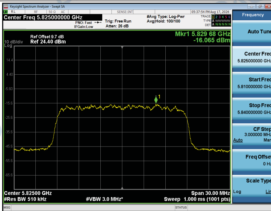
Power_Spectral_Density_NVNT_ANT2_802_11n(HT20)_5825
