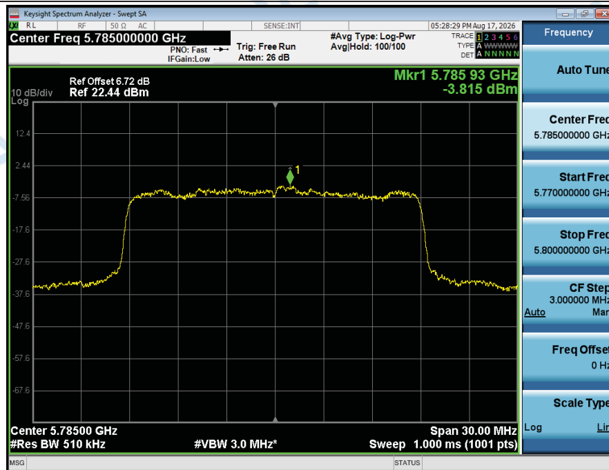
Power_Spectral_Density_NVNT_ANT2_802_11n(HT20)_5785
