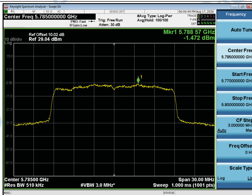
Power_Spectral_Density_NVNT_ANT2_802_11ac(VHT20)_5785
