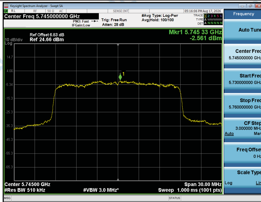
Power_Spectral_Density_NVNT_ANT2_802_11n(HT20)_5745
