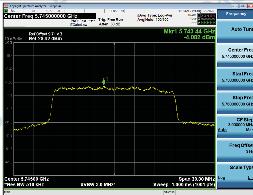
Power_Spectral_Density_NVNT_ANT2_802_11ac(VHT20)_5745
