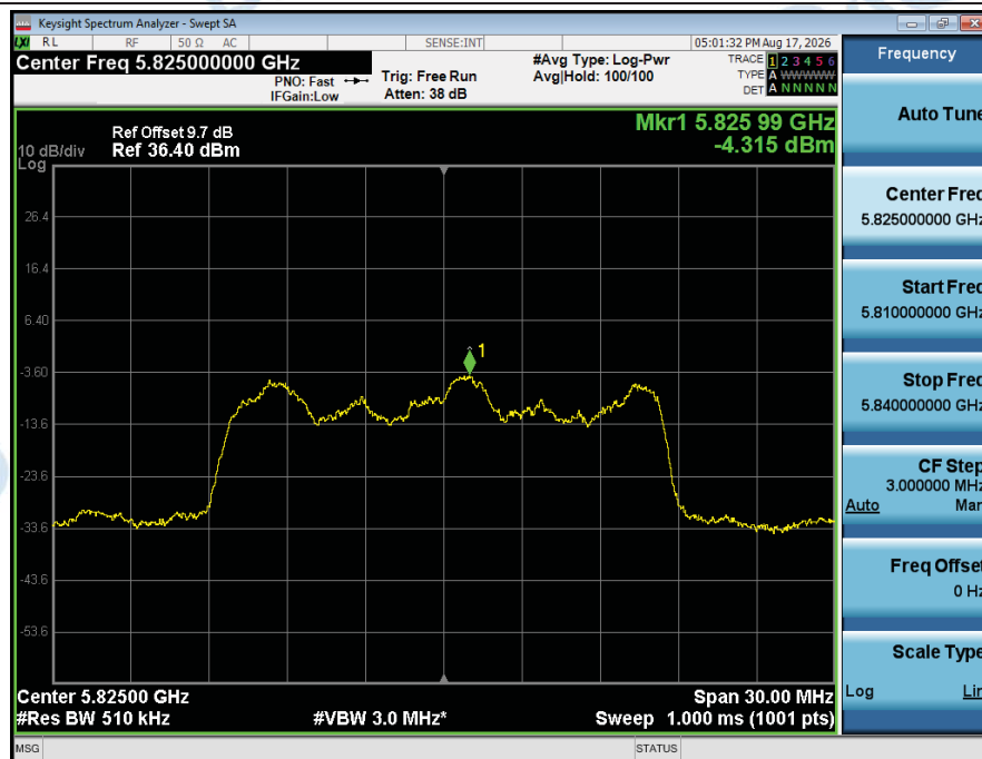
Power_Spectral_Density_NVNT_ANT2_802_11a_5825
