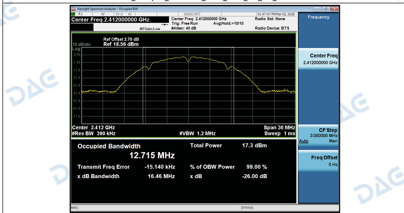
99%_Occupied_Bandwidth_NVNT_ANT1_802_11b_2412
