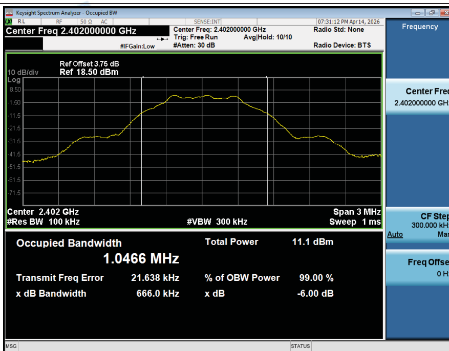
-6dB_Bandwidth_NVNT_ANT1_1Mbps_2402
