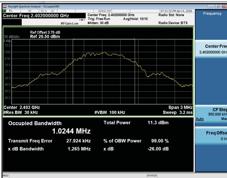
99%_Occupied_Bandwidth_NVNT_ANT1_1Mbps_2402
