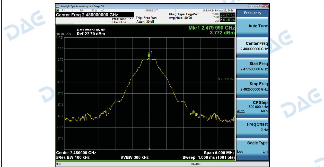
2_Spurious_Emissions_NVNT_ANT1_1-DH5_2480_00
