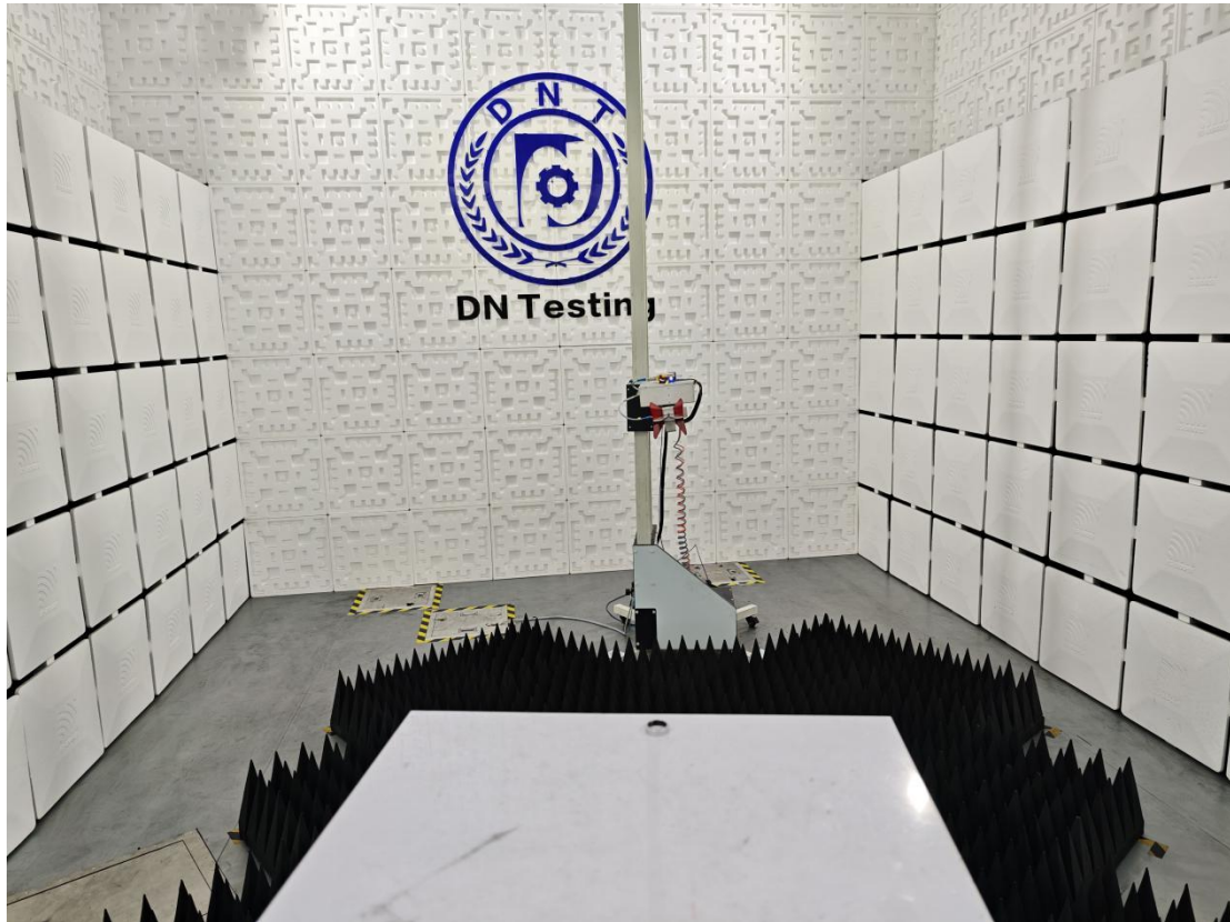
Radiated Emission Test View(Above 1G)
