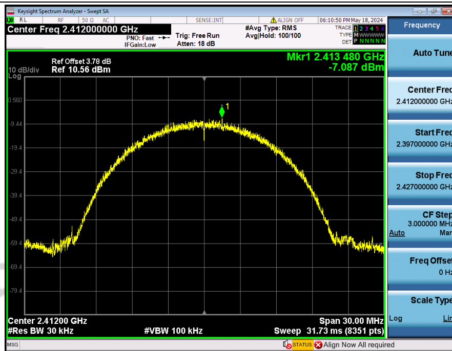
Power_Spectral_Density_NVNT_ANT1_802_11b_2412
