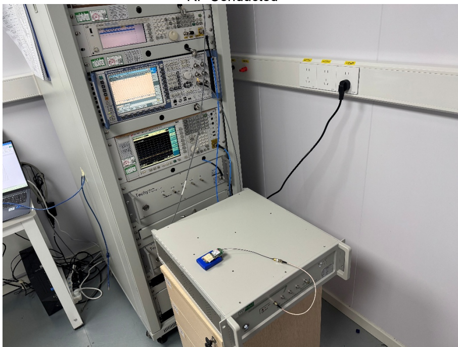
RF Conducted
